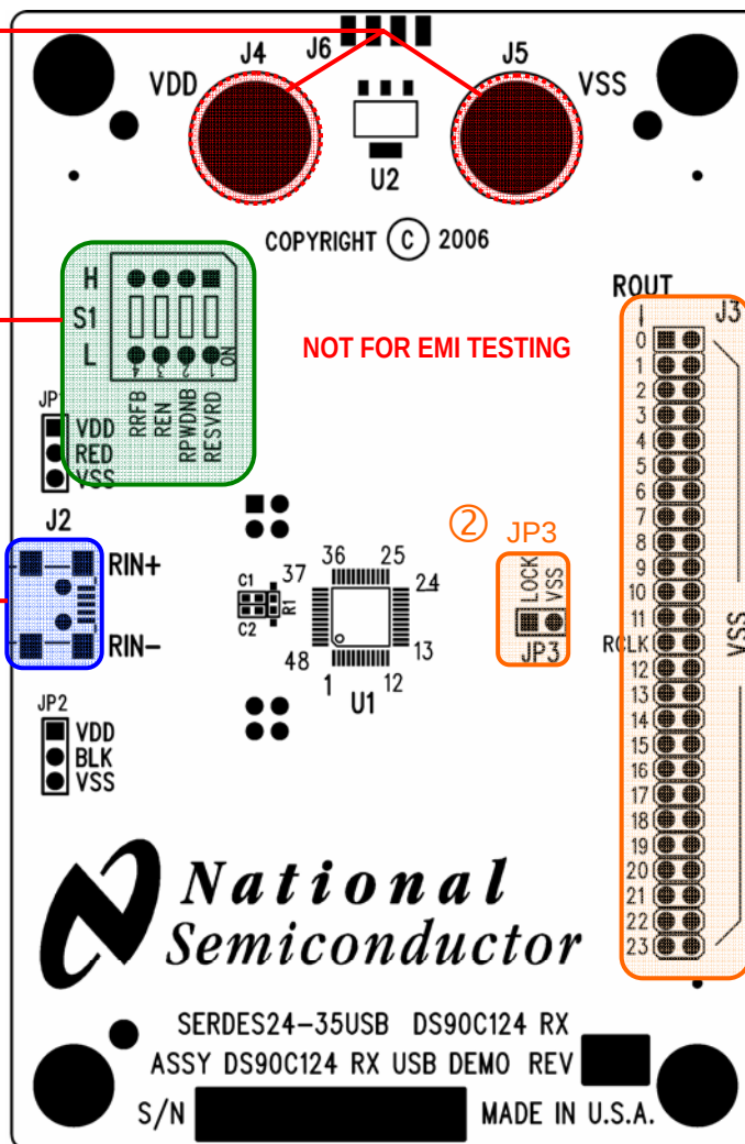
Figure 3. DS90C124 Rx Evaluation Board
