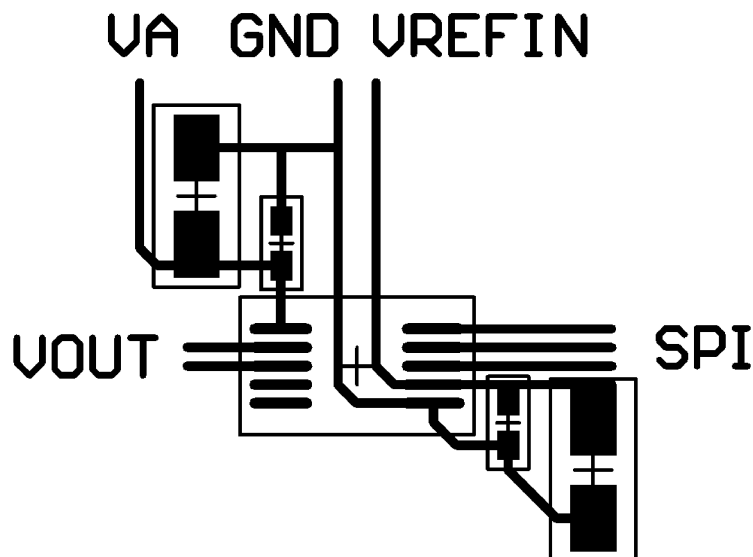
Figure 44. DAC102S085 Layout Diagram
