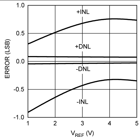
Figure 8. INL and DNL vs V_{REFIN} at V_A = 5 V
