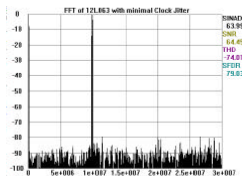
Figure 4b. Minimal clock jitter results in cleaner FFT, better dynamic performance
