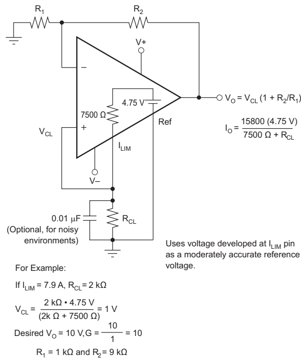
Figure 11. Voltage Source
