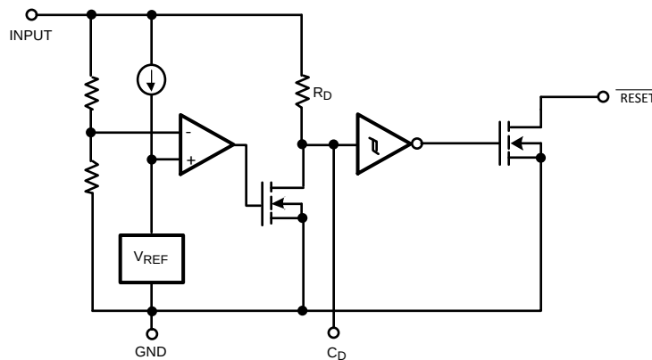
Figure 13. Open-Drain Output
