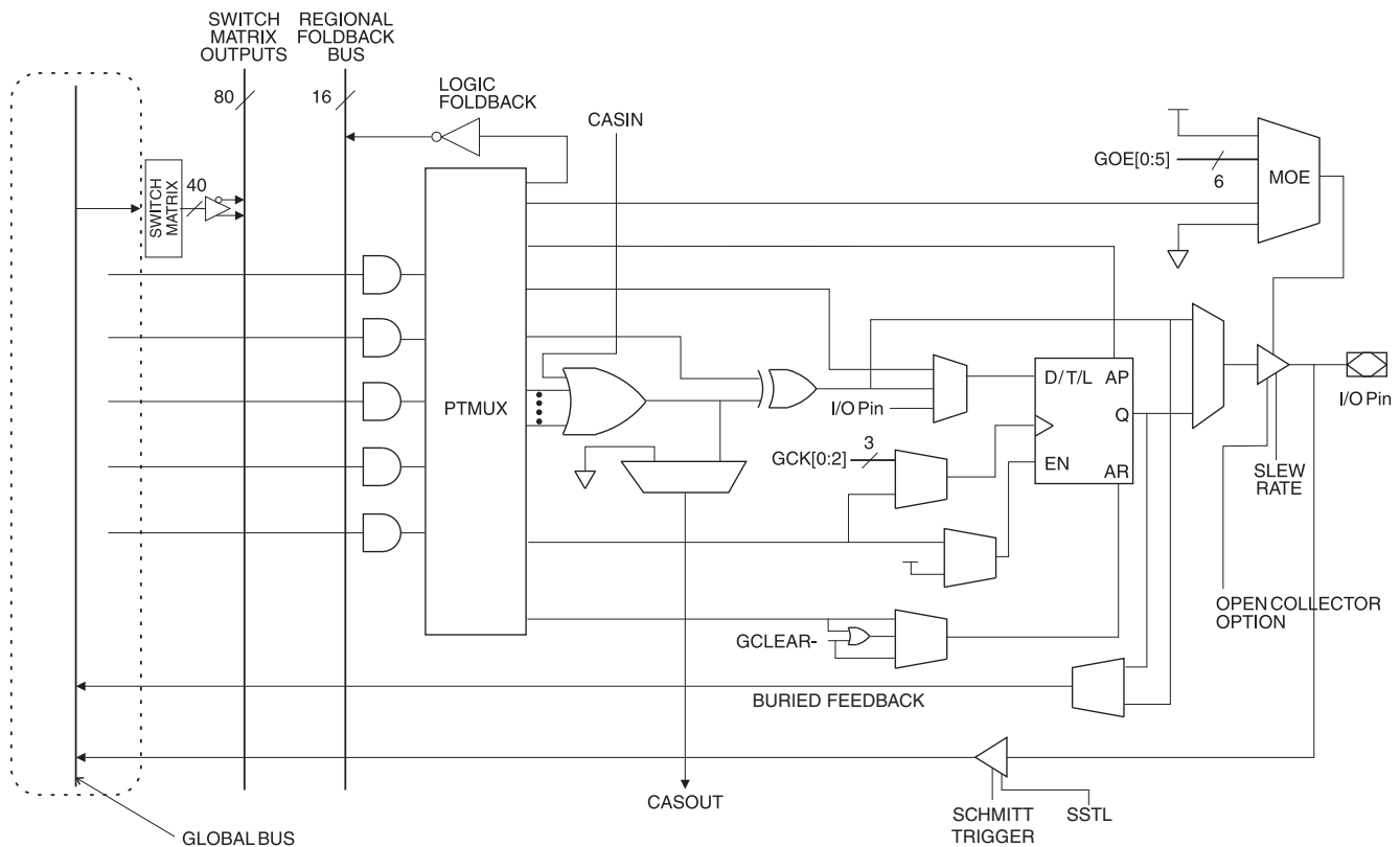
Figure 1-4. ATF1508RE Macrocell
