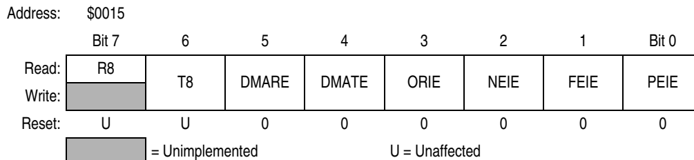
Figure 9-11. SCI Control Register 3 (SCC3)
