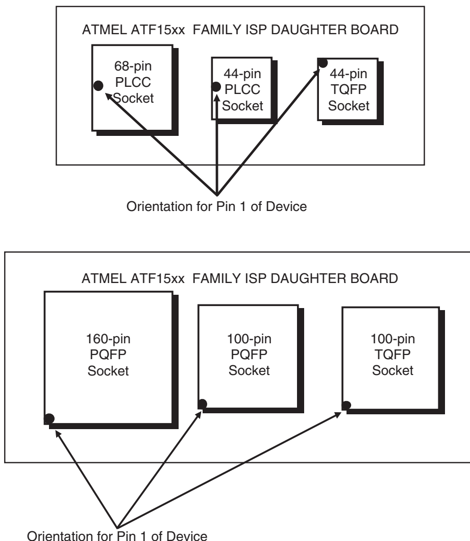
Figure 4-3. ISP Daughter Board
