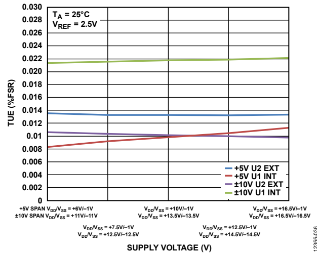
Figure 36. TUE vs. Supply Voltage
