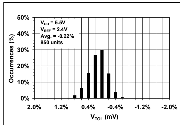
FIGURE 2-62: Reference Voltage Tolerance.
