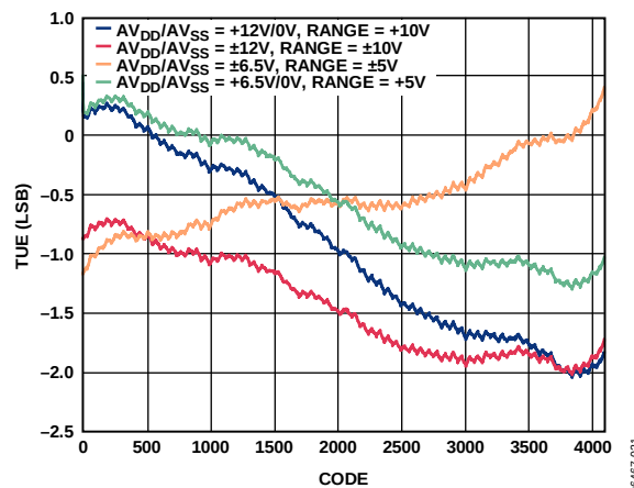
Figure 37. AD5722 Total Unadjusted Error vs. Code
