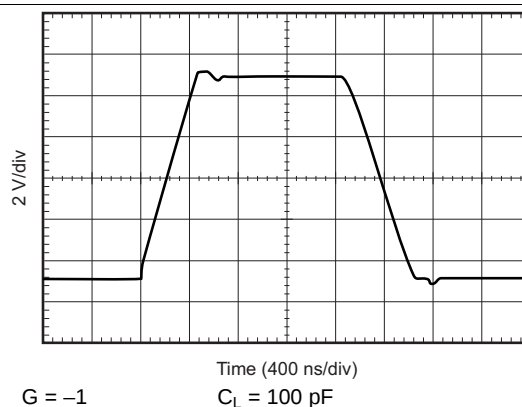
Figure 16. Large-Signal Step Response
