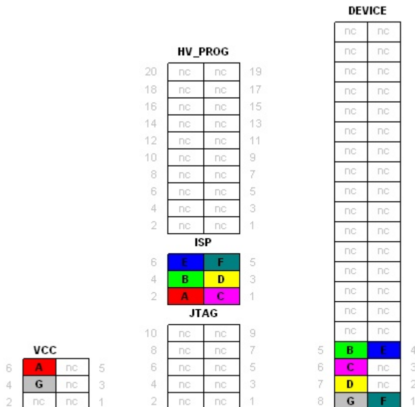
Figure 6-8. SPI Programming and debugWIRE Debugging
