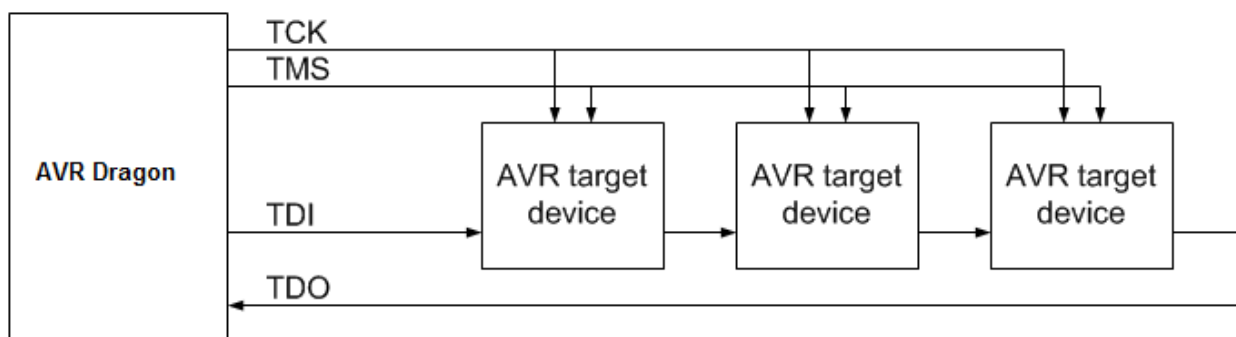
Figure 4-4. JTAG Daisy-chain
