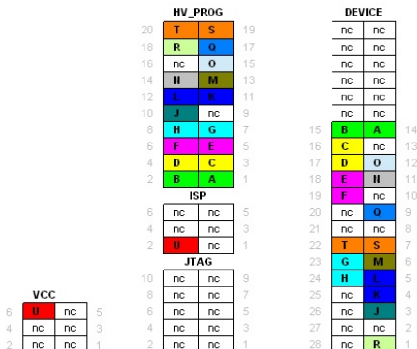
Figure 6-10. Parallel Programming
