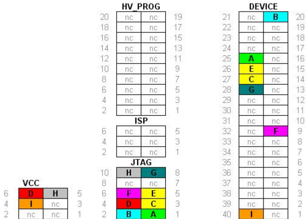
Figure 6-17. JTAG Programming and Debugging
