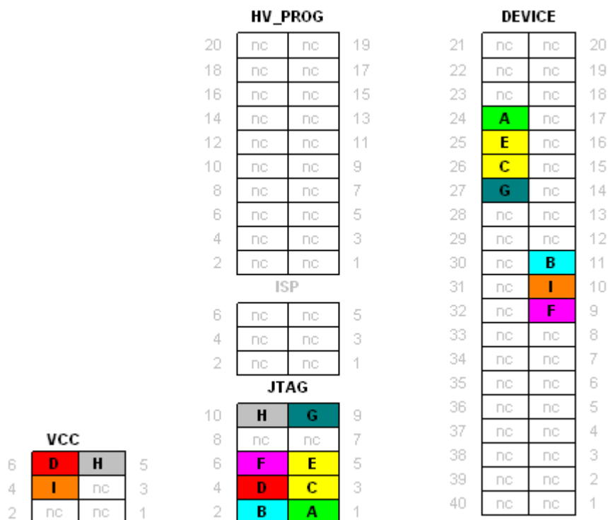
Figure 6-3. Parallel Programming
