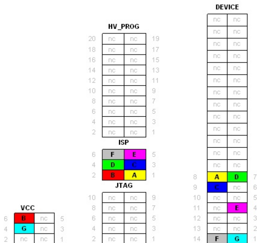
Figure 6-13. SPI Programming and debugWIRE Debugging
