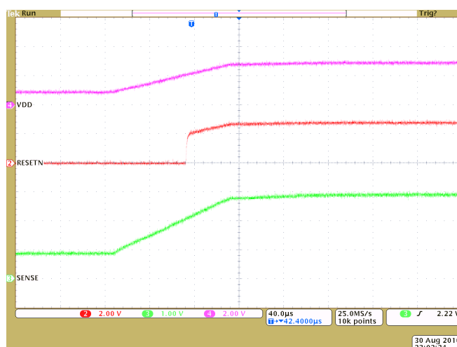
Figure 15. TPS3803-01-Q1 Low-to-High-Level Output
