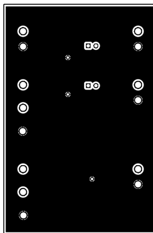
Figure 8. Bottom Layer
