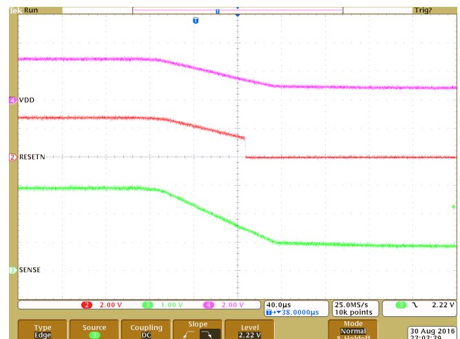
Figure 12. TPS3803-01-Q1 High-to-Low-Level Output
