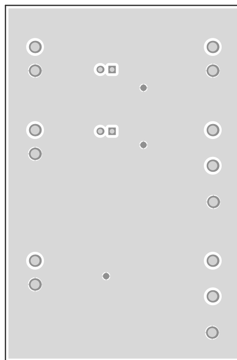
Figure 6. Layout—Bottom
