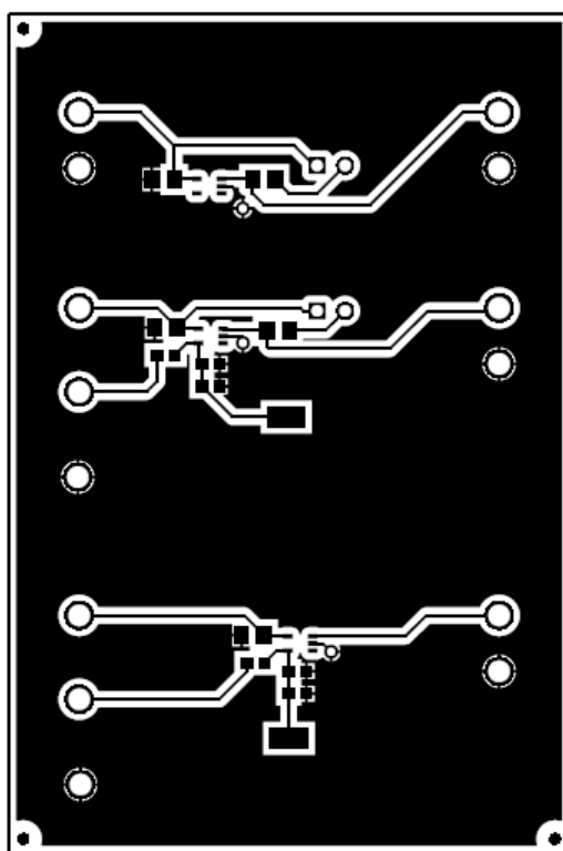
Figure 7. Top Layer
