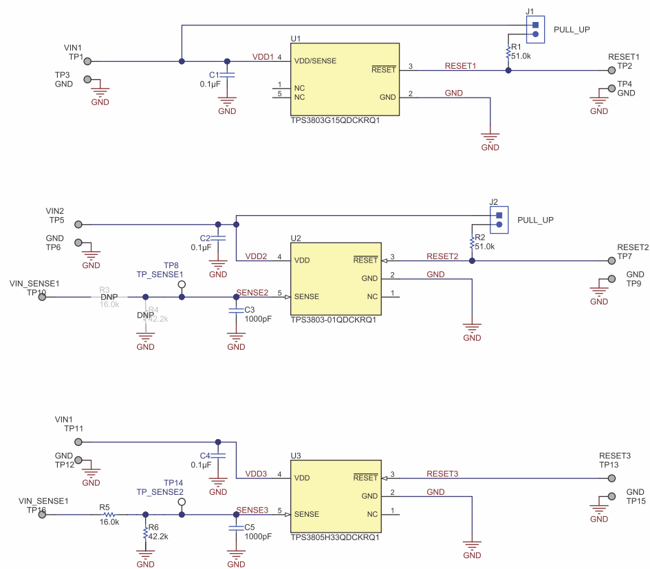
Figure 2. TPS3803X-Q1EVM Schematic
