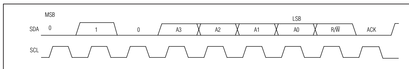
Figure 9. Slave Address
