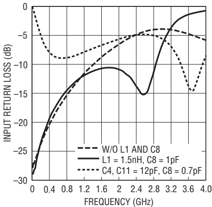
Figure 2. Input Return Loss with Additional LC Matching Network
