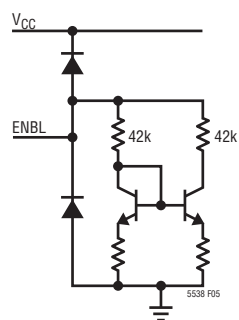
Figure 5. Simplified Schematic of the Enable Circuit
