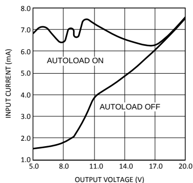
Figure 7. Auto-Load Effect on Input Current, No Load
