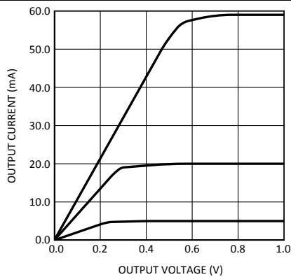
Figure 3. V_{SAT} vs I_{LED}
