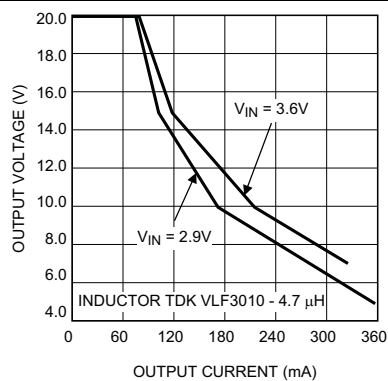
Figure 5. Boost Maximum Output Voltage vs Current
