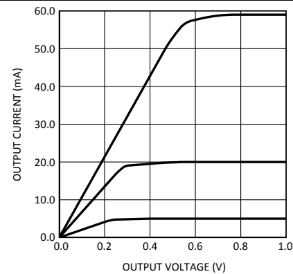
Figure 4. V_{SAT} vs I_{LED}
