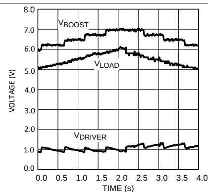
Figure 8. Adaptive Output Voltage Operation
