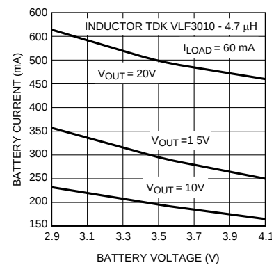
Figure 6. Battery Current vs Voltage
