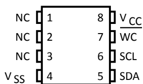
Figure 2. 8-pin package connections, top view
