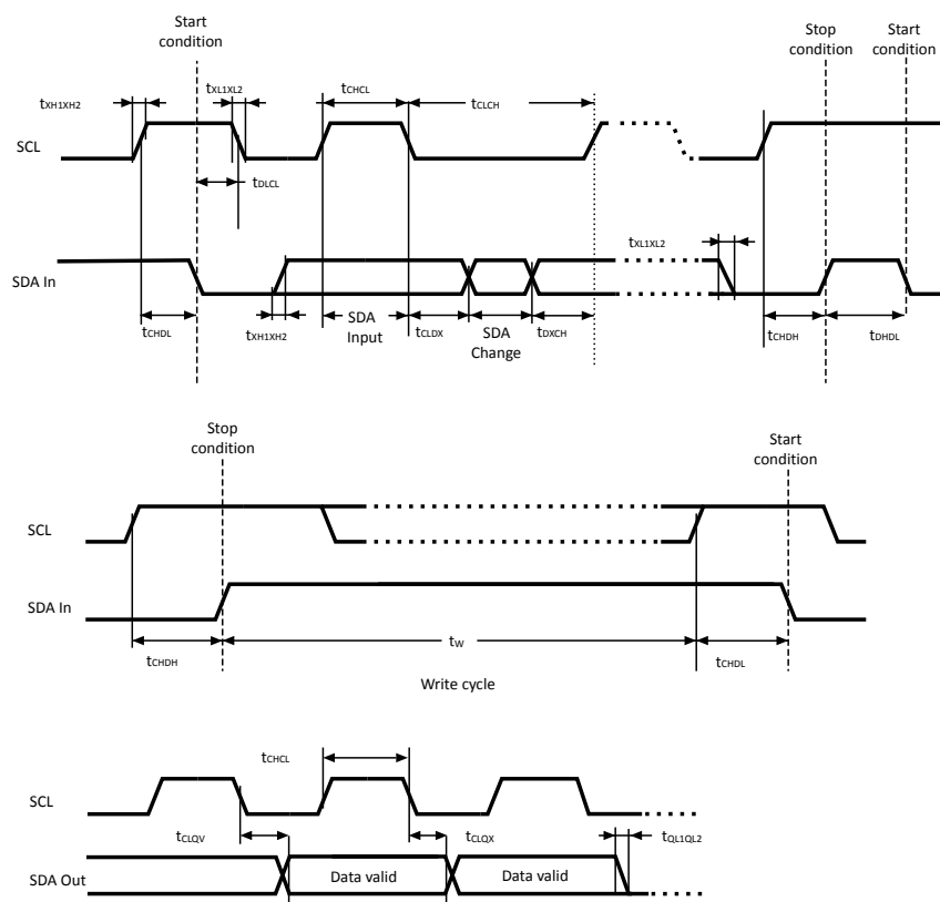
Figure 12. AC waveforms
