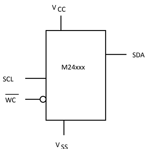
Figure 1. Logic diagram
