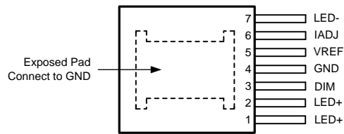
Figure 6. 7-Pin PFM (Top View) See NDW0007A Package
