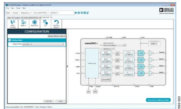
Figure 3. Chip Block Diagram View for the AD5676R
