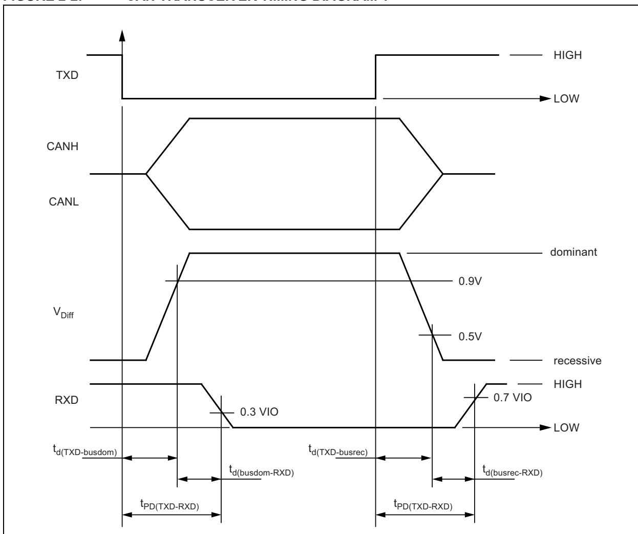
FIGURE 2-2: CAN TRANSCEIVER TIMING DIAGRAM 1
