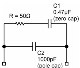
Figure 4. Loop Filter
