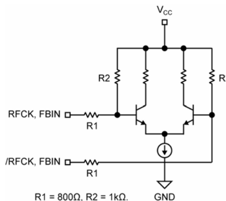
Figure 10. Simplified Input Structure
