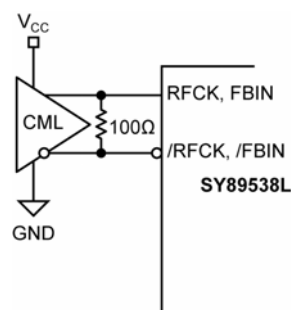
Figure 11c. CML Interface (DC-Coupled)
