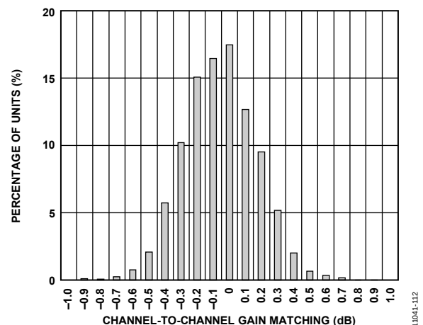
Figure 14. Gain Matching Histogram, V_{\text{GAIN}} = 1.2 V
