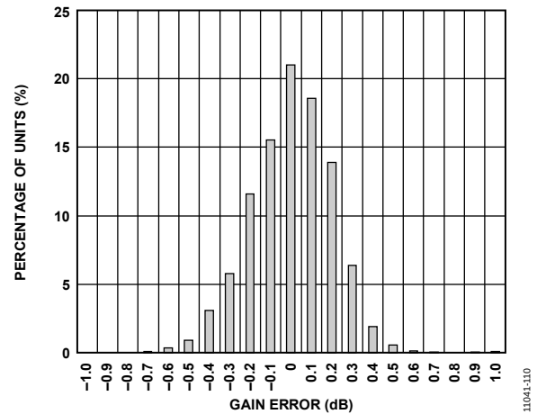
Figure 12. Gain Error Histogram, V_{\text{GAIN}} = 1.28 V
