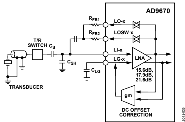
Figure 37. Simplified LNA Input Configuration
