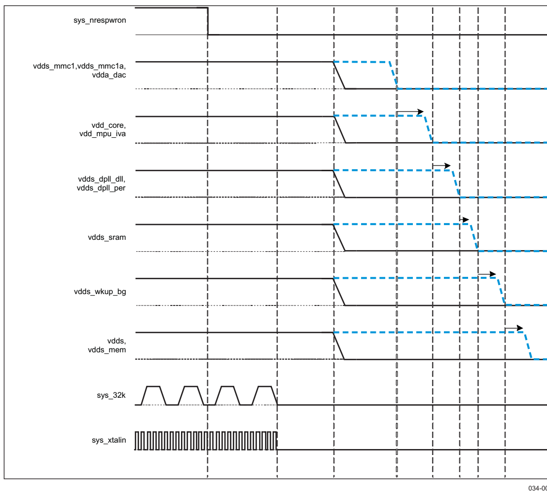
Figure 3-4. Power-down Sequence
