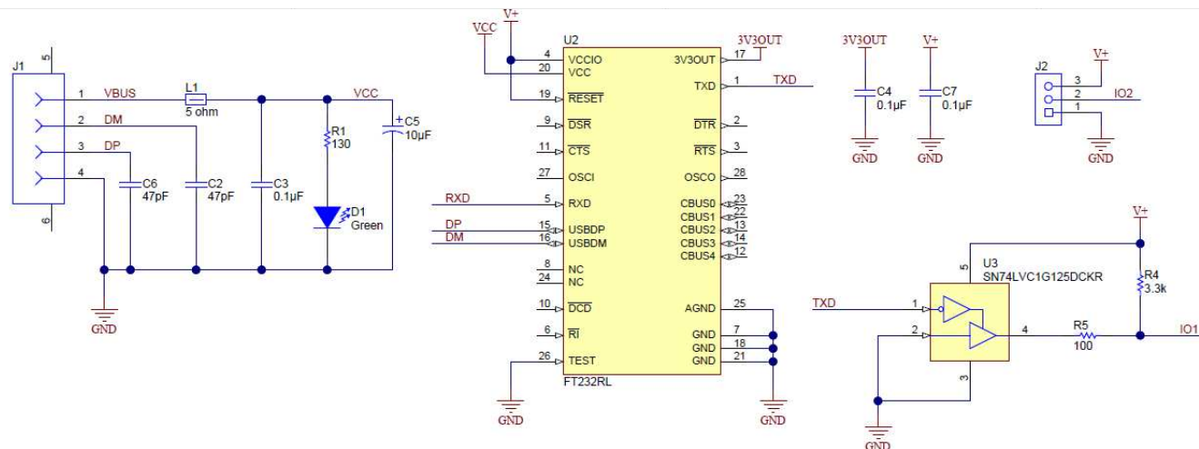
Figure 19. TMP107EVM Schematic
