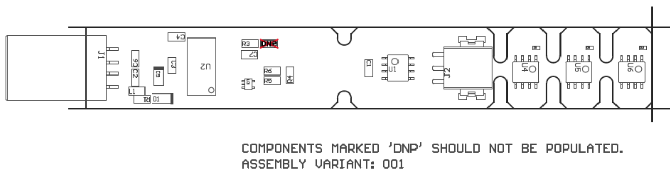
Figure 21. TMP107EVM PCB Assembly Drawing
