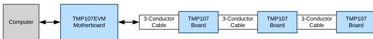
Figure 2. TMP107EVM System Setup
