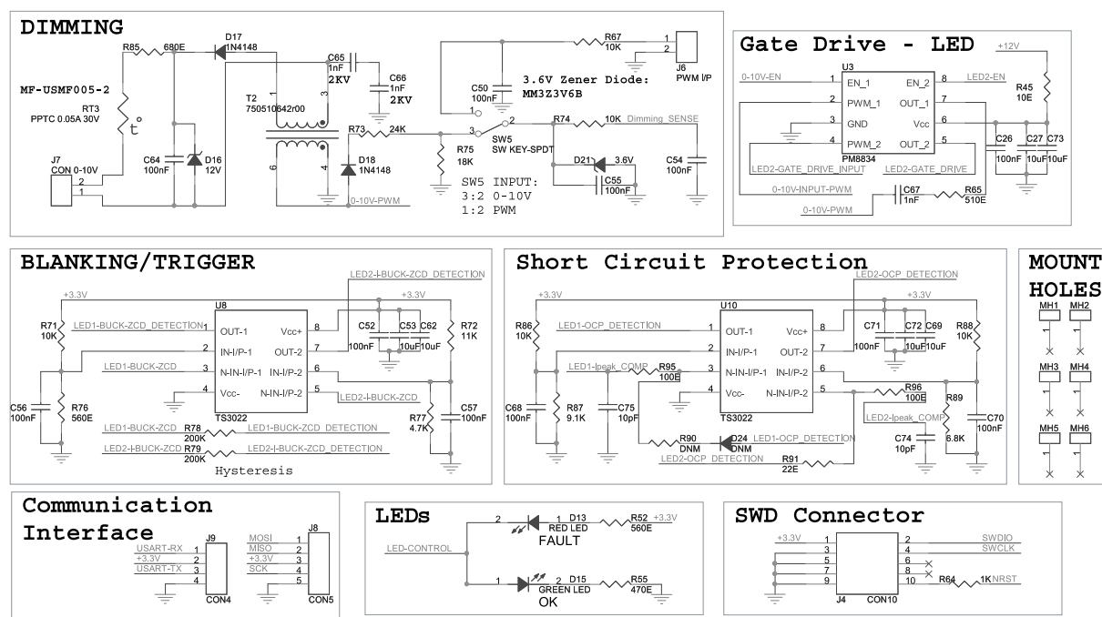
Figure 7. STEVAL-LLL004V1 schematic - miscellaneous
