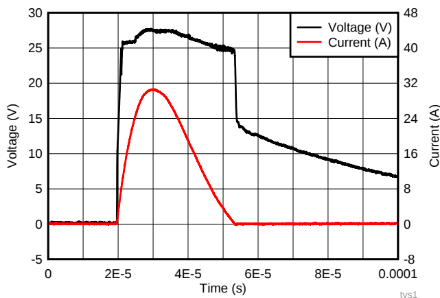
Figure 8. Surge Waveform at 30 A
