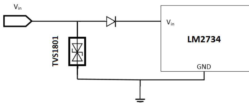
Figure 7. TVS1801 Application Schematic
