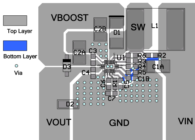
Figure 3: Layout Recommendation
