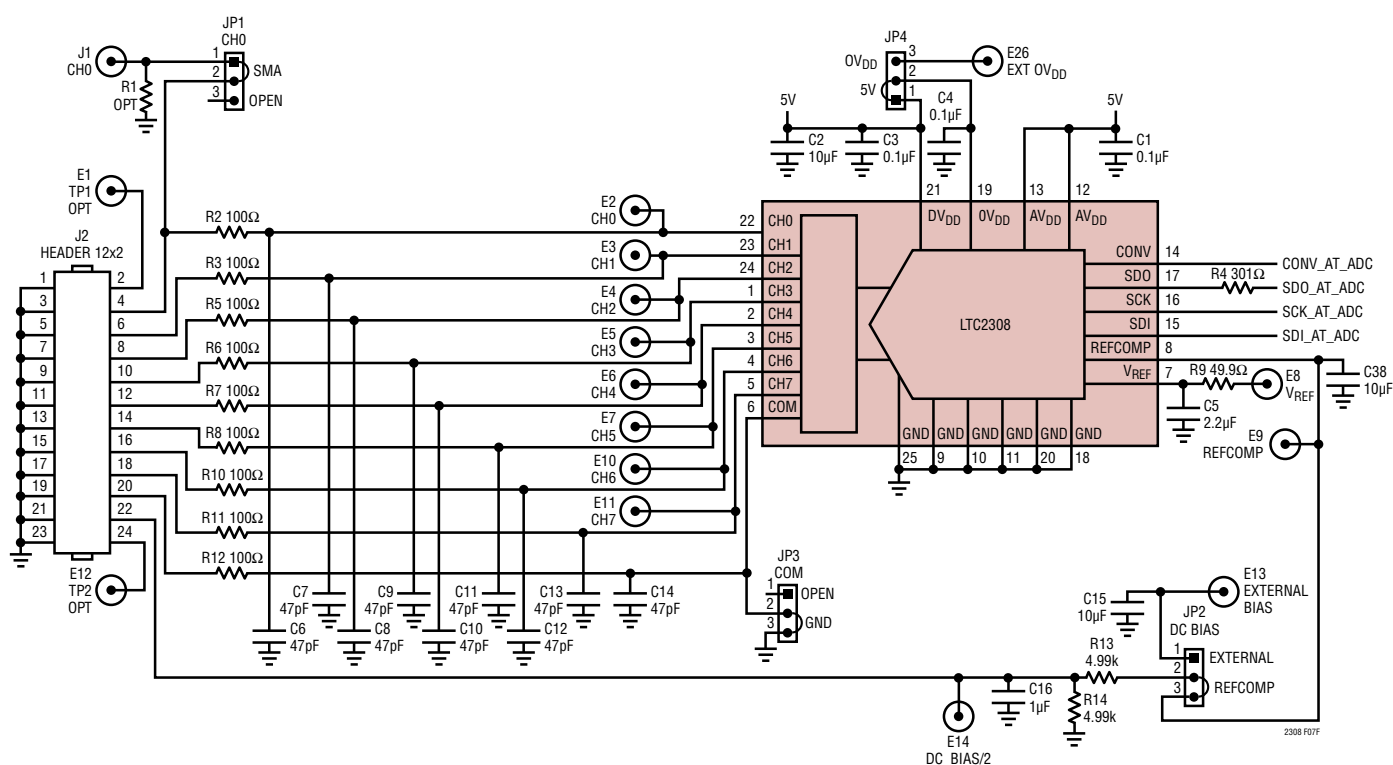
Figure 7f. Partial Demo Board Schematic
