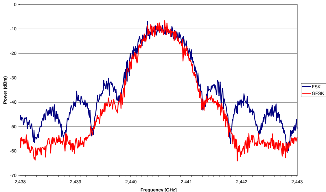
Figure 18. Modulated spectrum
