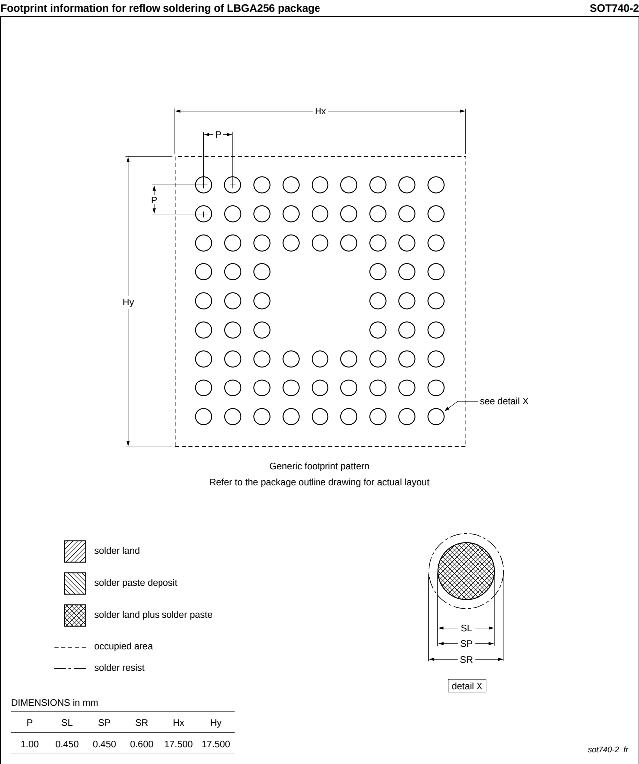
Fig 53. Reflow soldering of the LBG256 package
