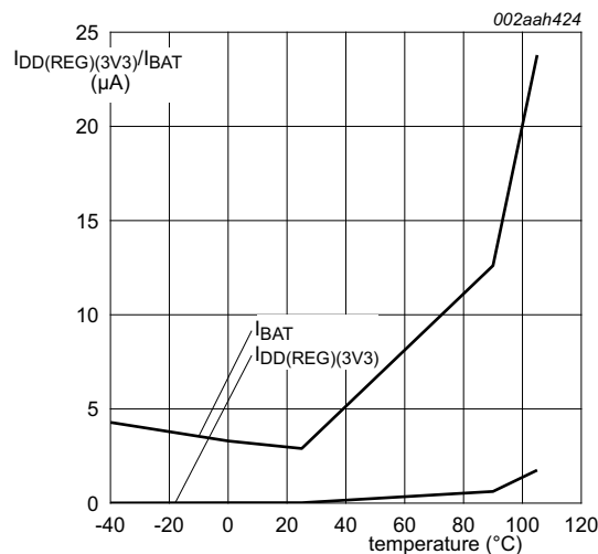
Fig 16. Typical supply current versus temperature in Deep power-down mode
