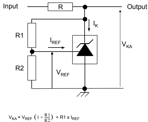
Figure 8. Test circuit for programming mode
