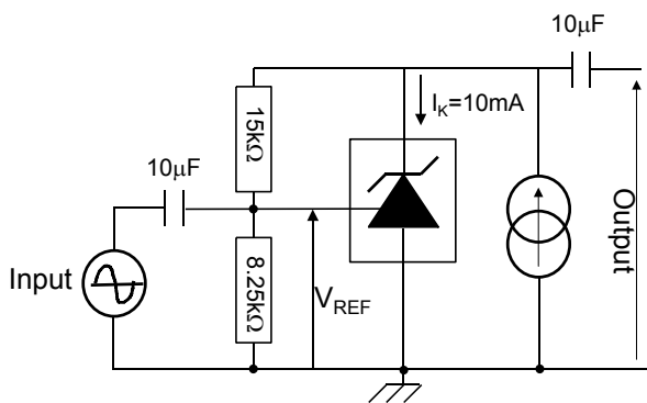
Figure 10. Test circuit for phase margin and voltage gain
