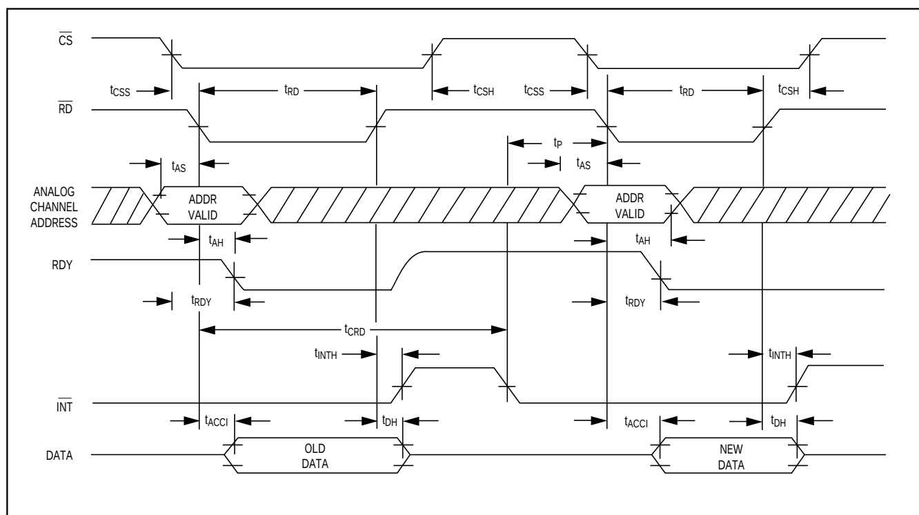
Figure 6. Mode 1 Timing Diagram
