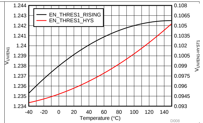
Figure 8. Enable/UV Threshold
