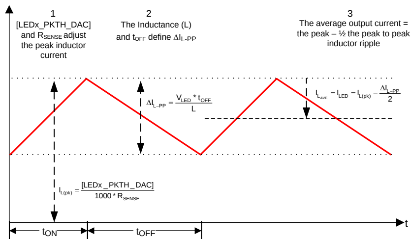
Figure 16. Hysteretic Operation
