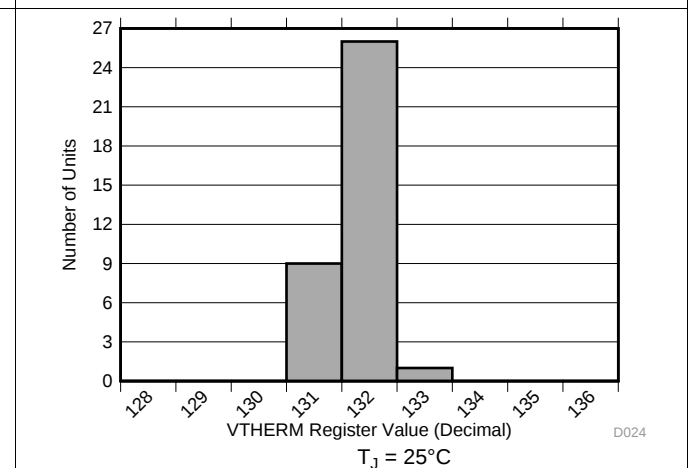
Figure 12. VTHERM Performance
