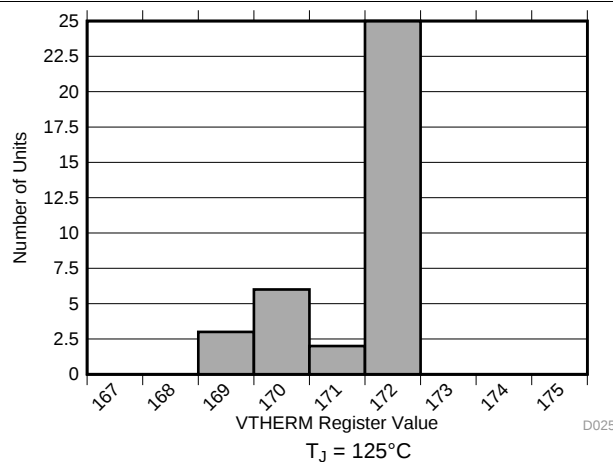
Figure 13. VTherm Performance
