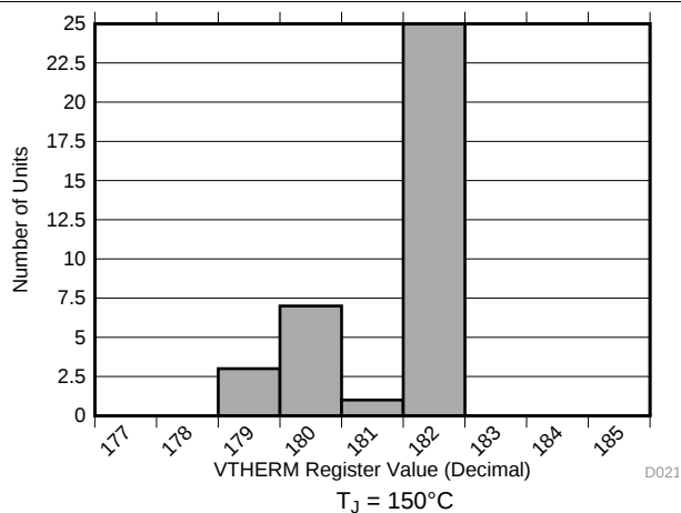
Figure 14. VTherm Performance
