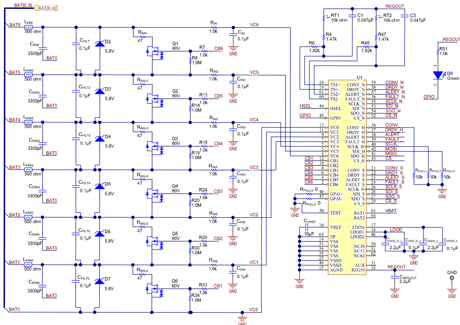
Figure 57. Application Schematic
