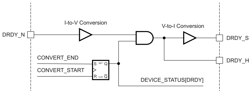
Figure 16. Data-Ready Logic
