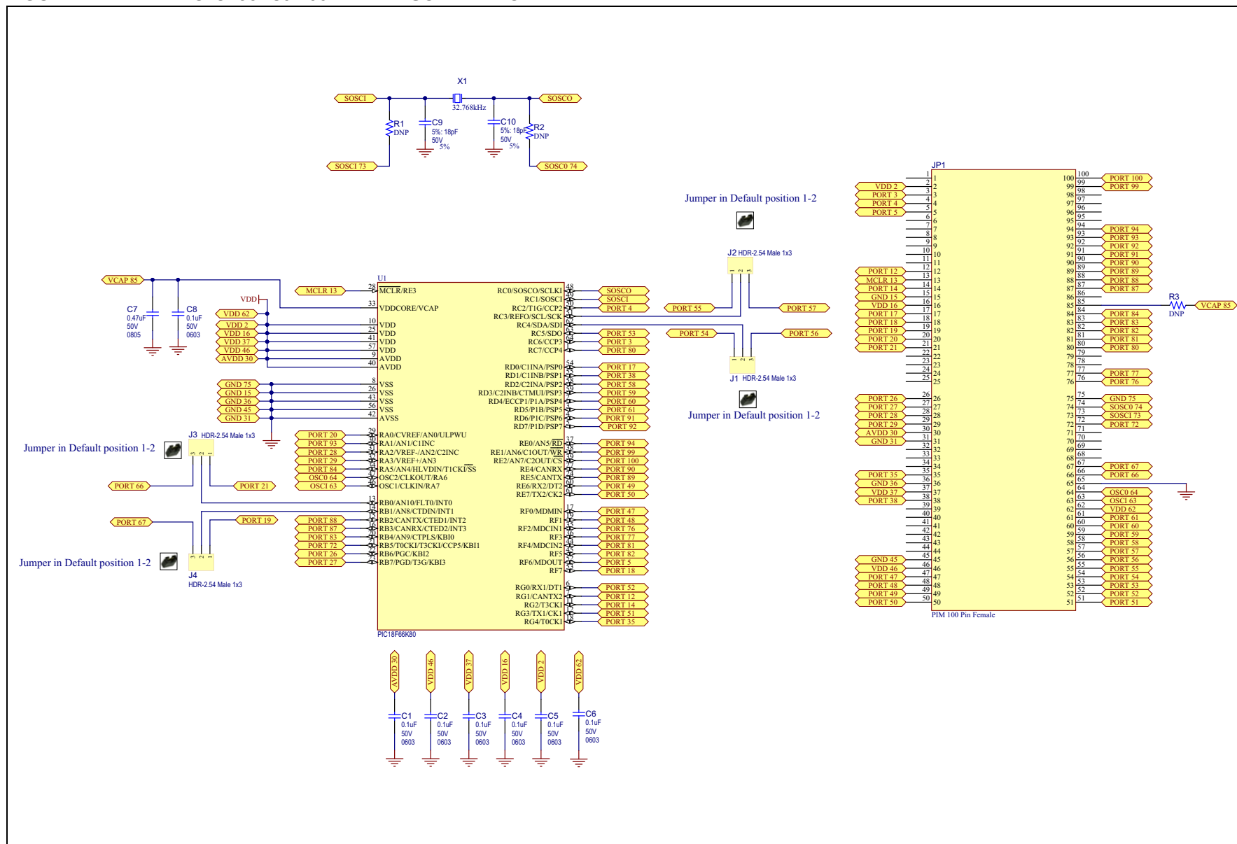
FIGURE A-1: PIC18F66K80 100-PIN PIM SCHEMATIC
