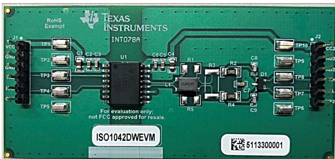
Figure 3. ISO1042DWEVM Photograph
