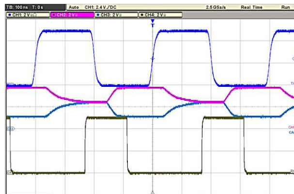
Figure 7. Typical Input and Output Waveforms
