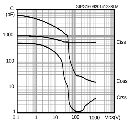
Figure 12: Capacitance variation
