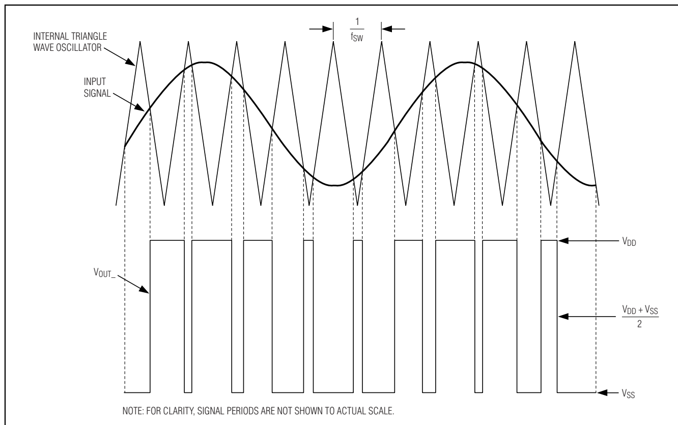
Figure 3a. MAX9742 Output with an Applied Input Signal
