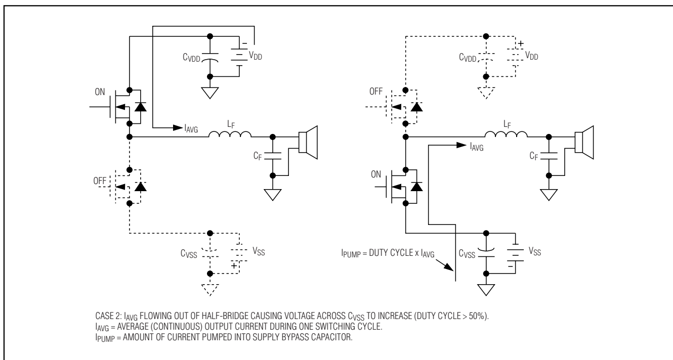
Figure 13b. Continuous Output Current Flow for Negative Supply Pumping
