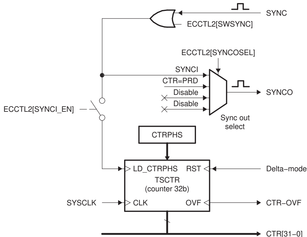
Figure 15-7. Details of the Counter and Synchronization Block
