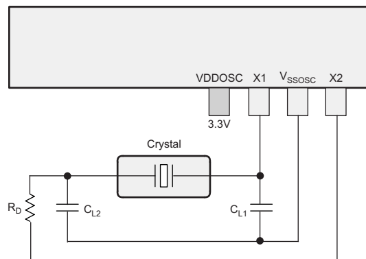
Figure 3-7. External Crystal
