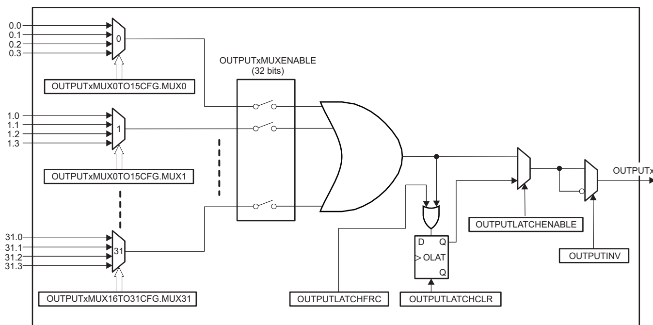
Figure 8-4. GPIO Output X-BAR Architecture
