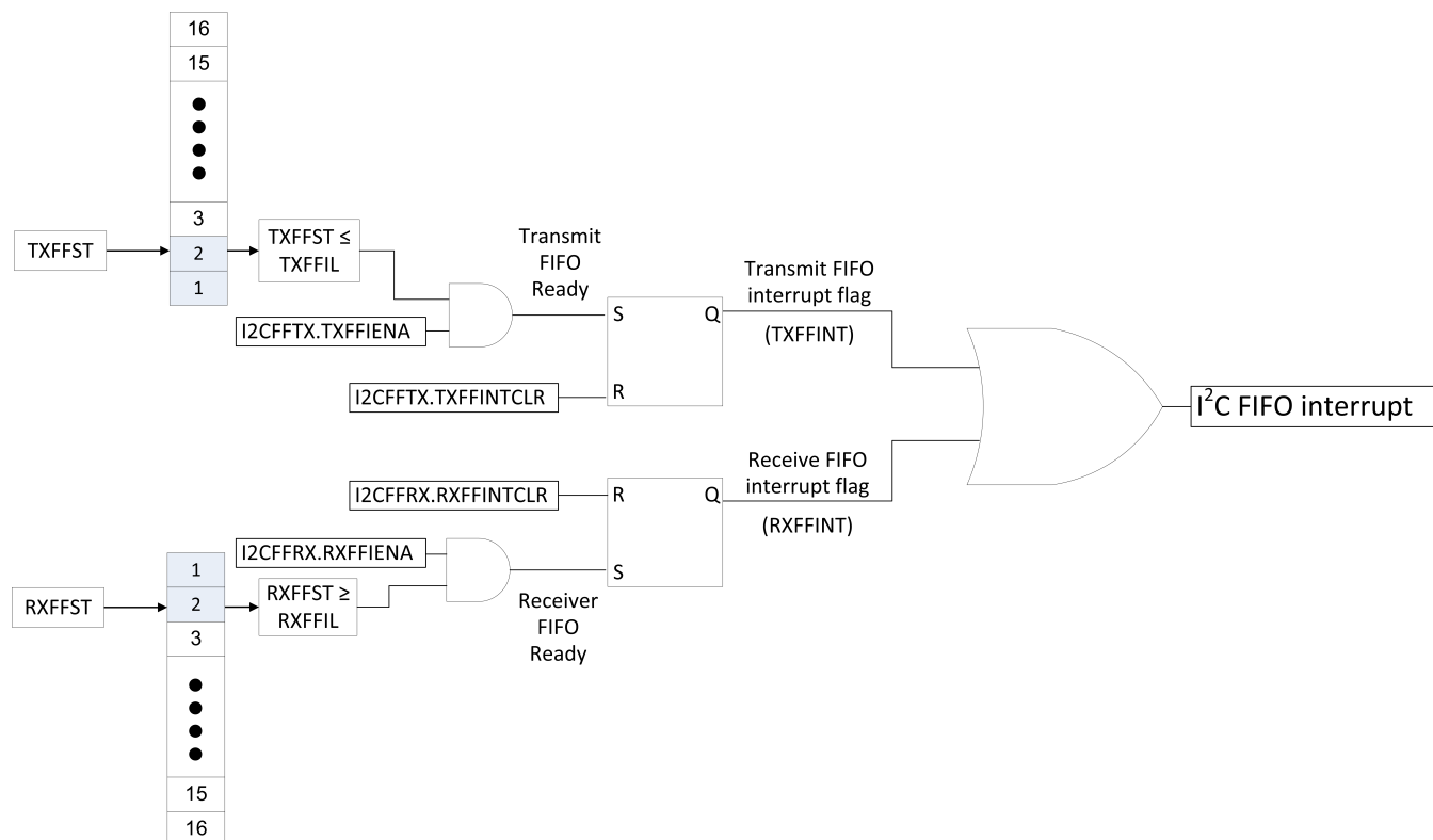
Figure 19-17. I2C_FIFO_interrupt
