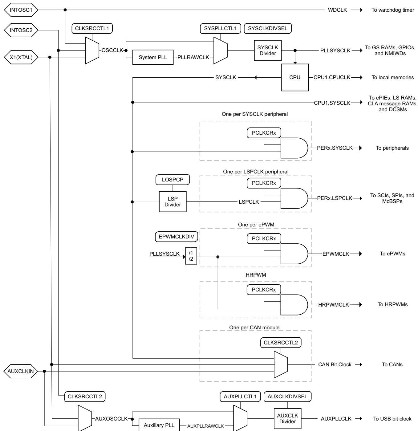
Figure 3-5. Clocking System
