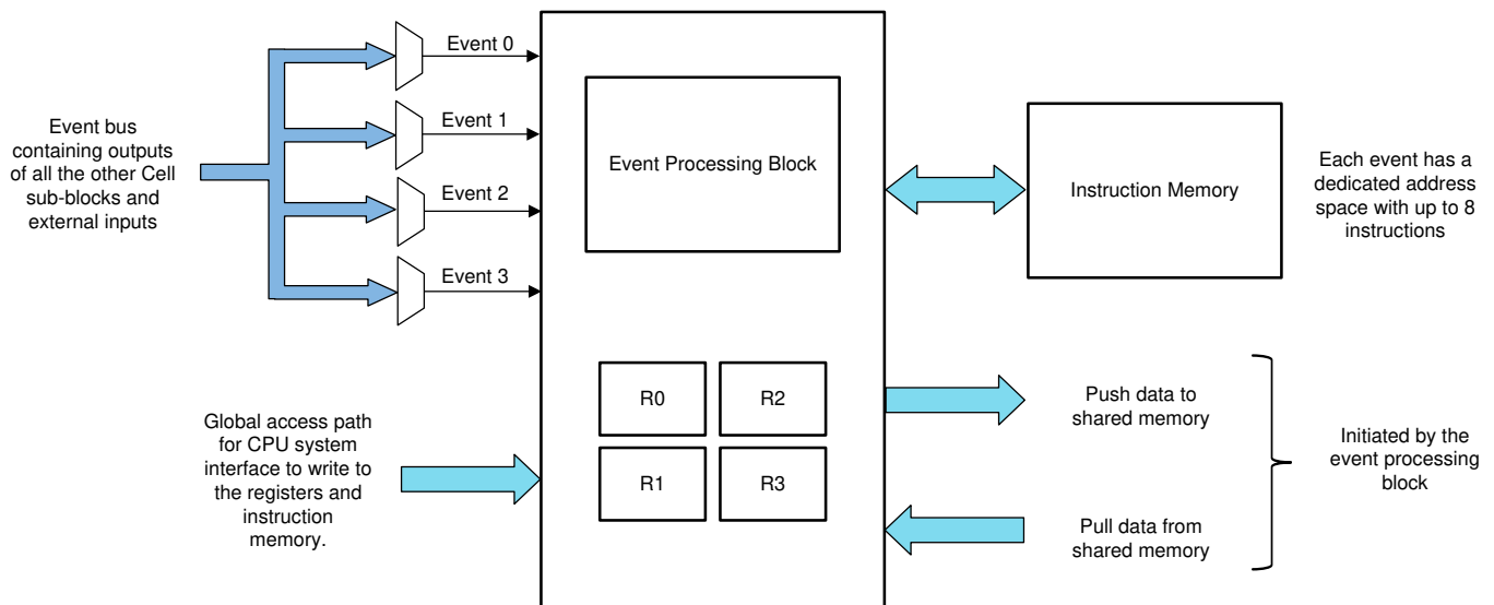
Figure 24-13. High Level Controller Block
