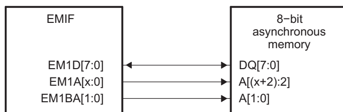
Figure 23-9. EMIF to 8-bit/16-bit Memory Interface
