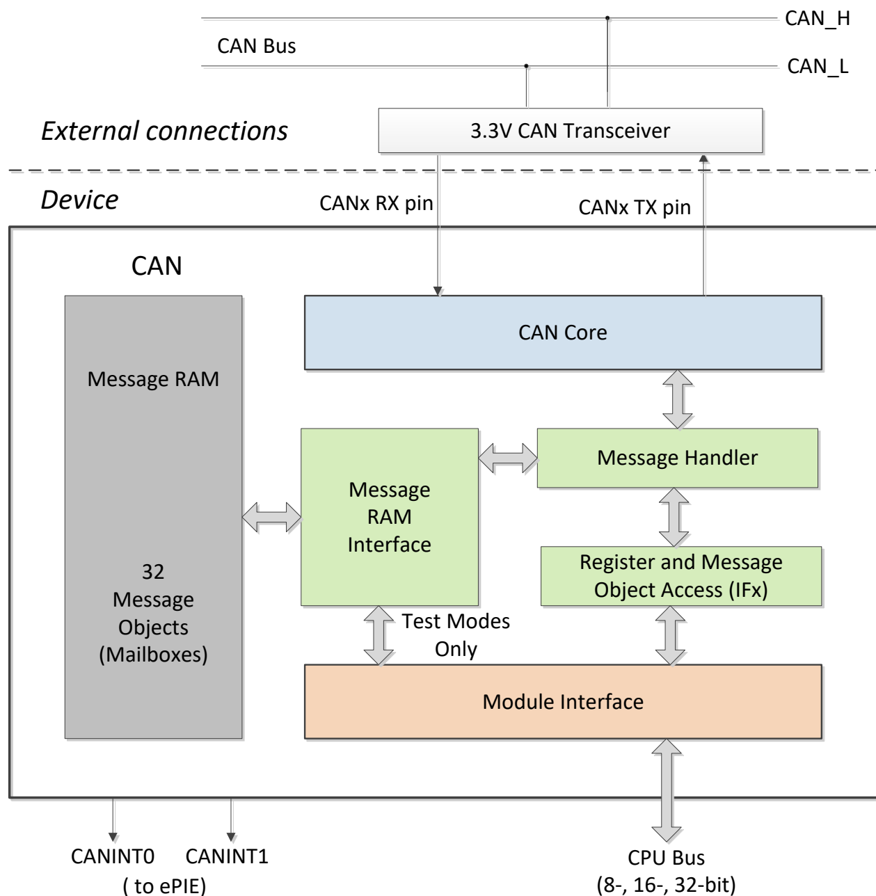
Figure 21-1. CAN Block Diagram
