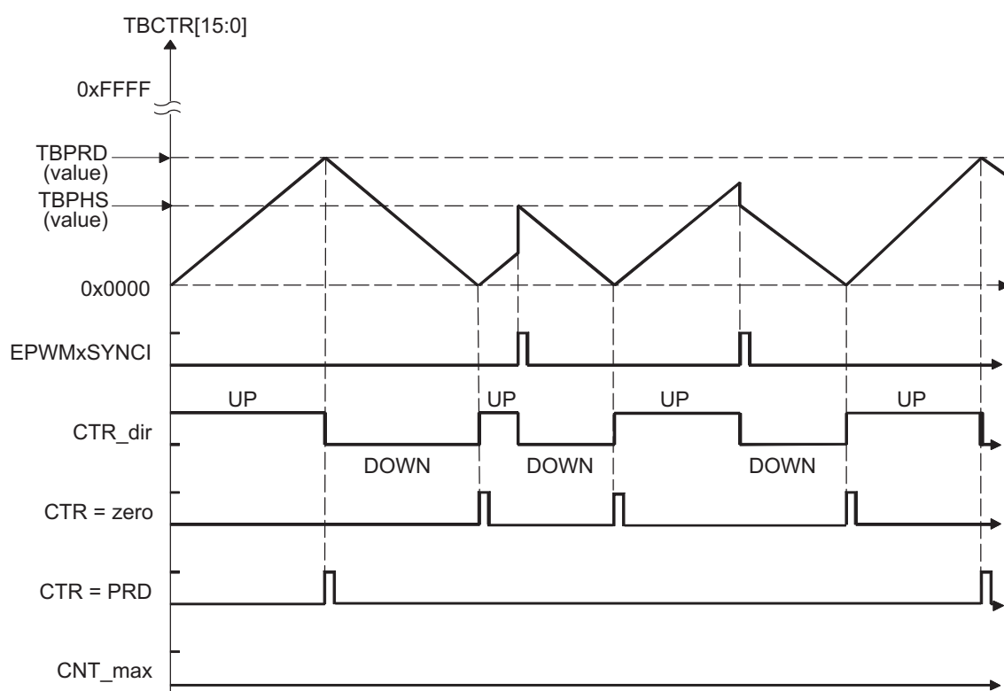
Figure 14-10. Time-Base Up-Down-Count Waveforms, TBCTL[PHSDIR = 0] Count Down On Synchronization Event
