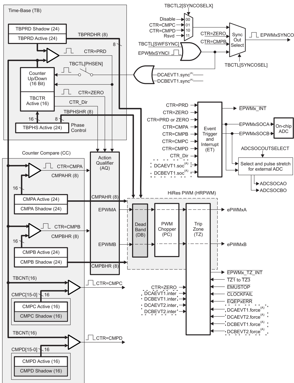
Figure 14-3. ePWM modules and Critical Internal Signal Interconnects
