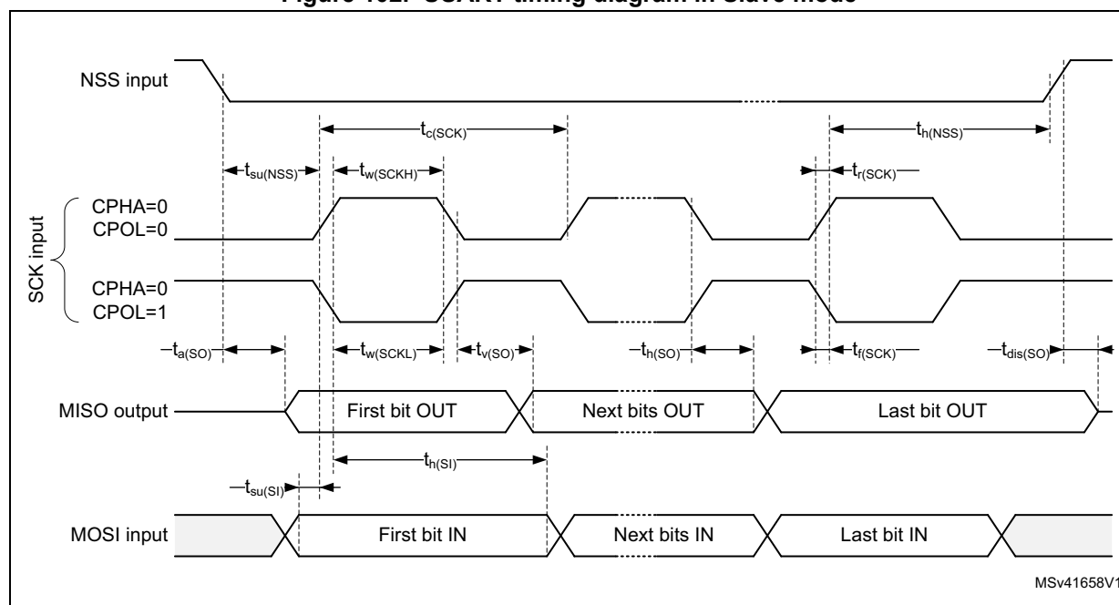
Figure 102. USART timing diagram in Slave mode
