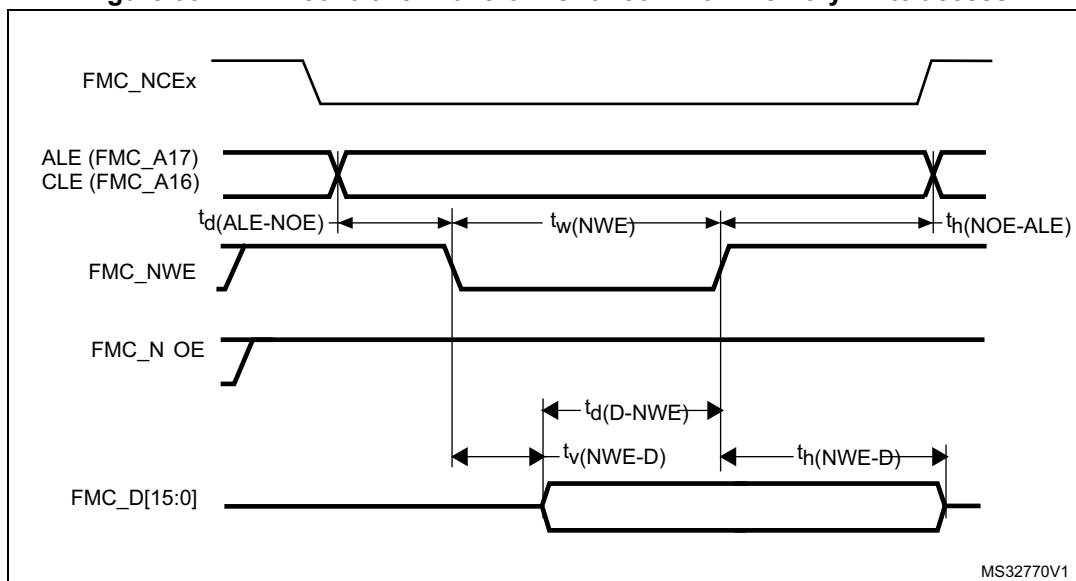
Figure 35. NAND controller waveforms for common memory write access
