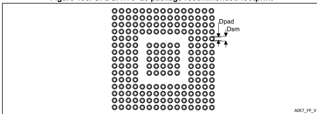
Figure 138. UFBGA176+25 package recommended footprint
