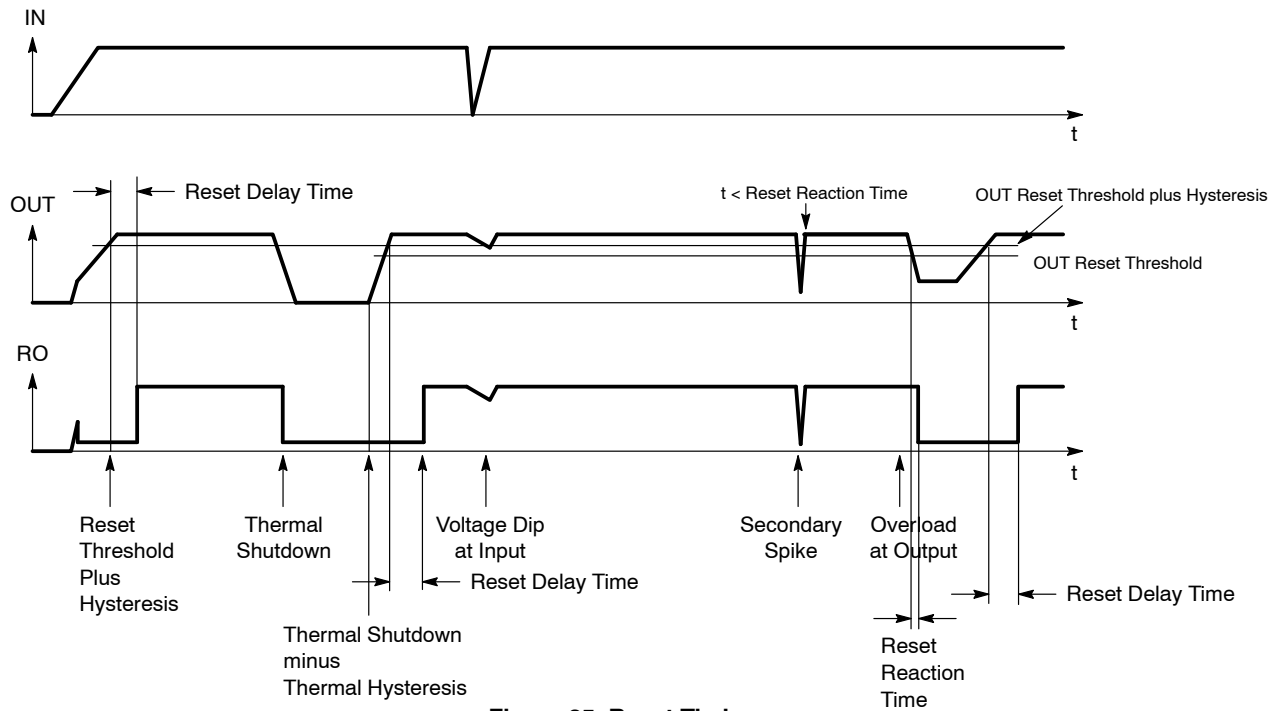
Figure 25. Reset Timing
