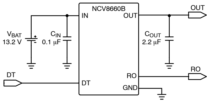
Figure 1. Application Diagram
