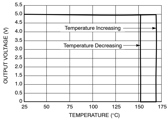
Figure 23. Thermal Shutdown vs. Temperature
