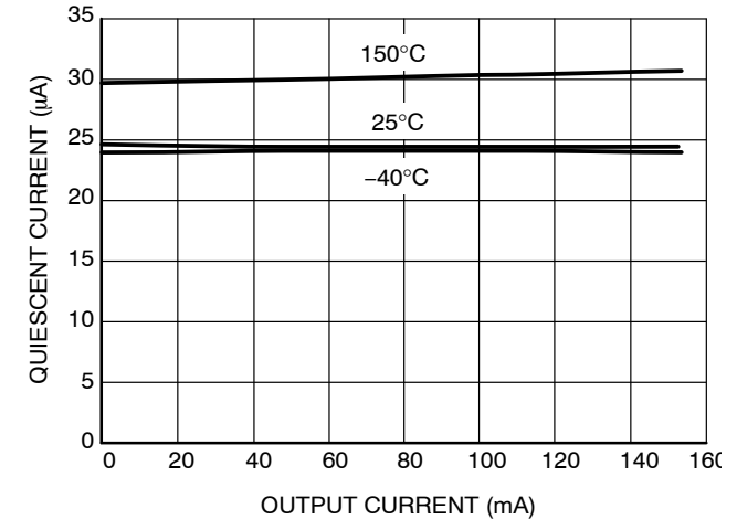
Figure 14. Quiescent Current vs. Output Current
