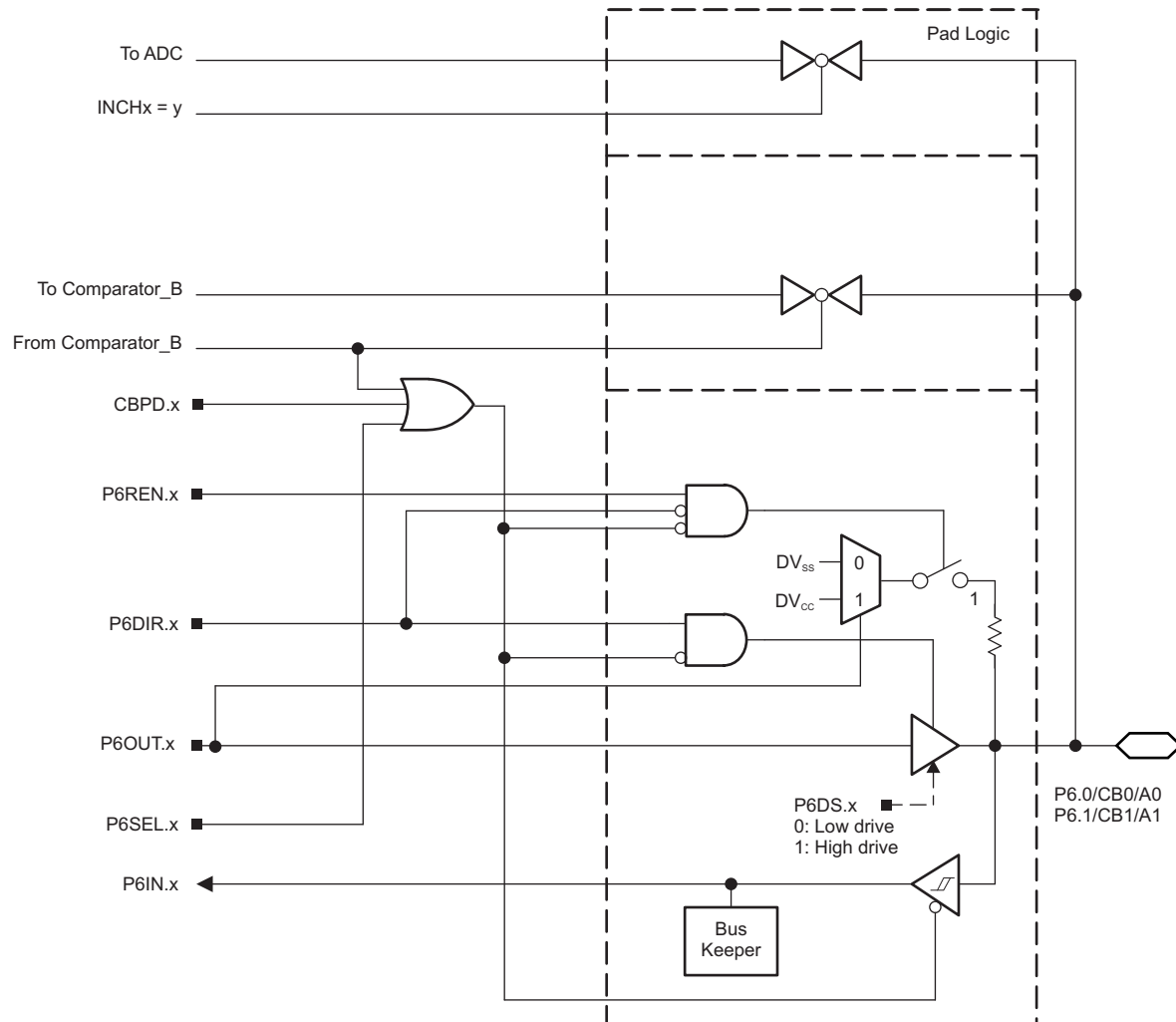
Figure 6-10. Port P6 (P6.0 to P6.1) Diagram
