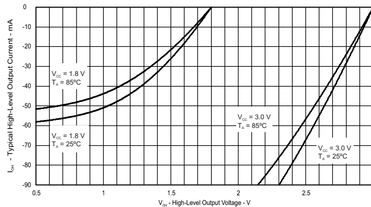
Figure 5-31. Ports PU.0, PU.1 Typical High-Level Output Characteristics
