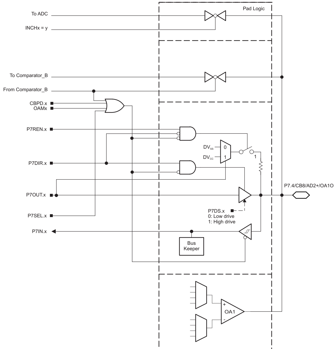
Figure 6-18. Port P7 (P7.4) Diagram
