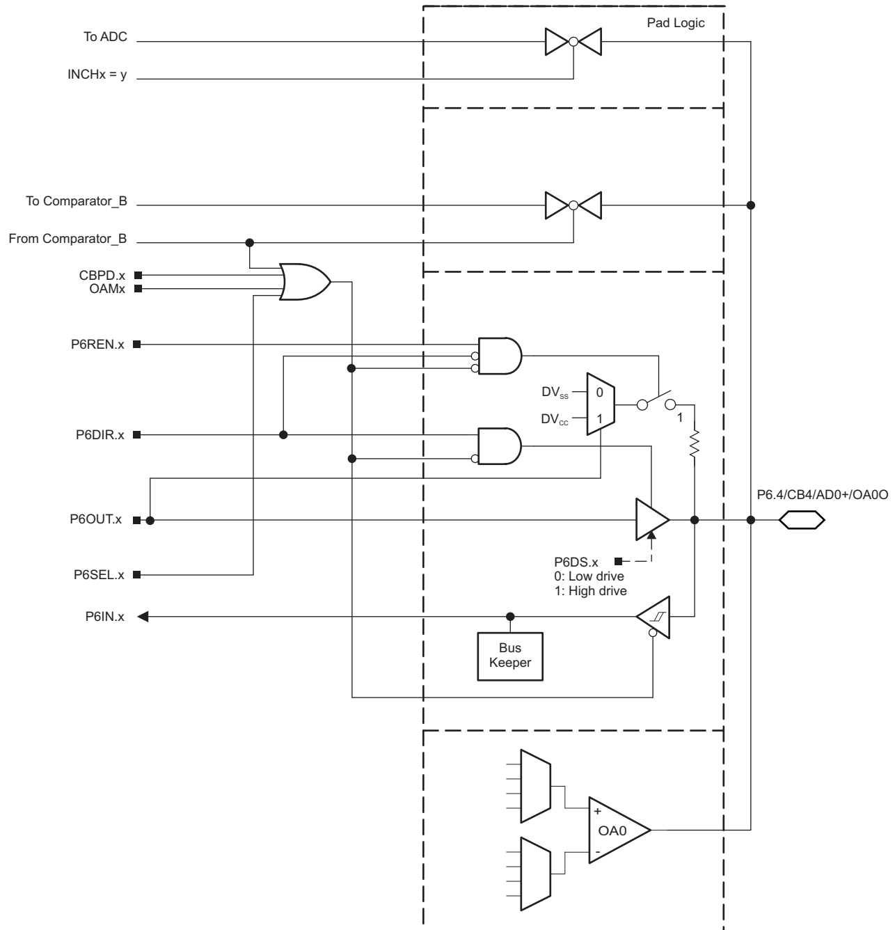
Figure 6-12. Port P6 (P6.4) Diagram
