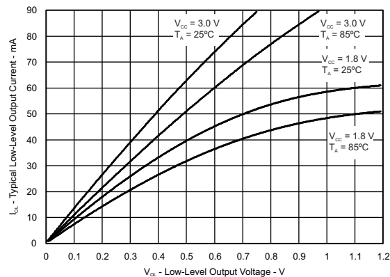
Figure 5-30. Ports PU.0, PU.1 Typical Low-Level Output Characteristics
