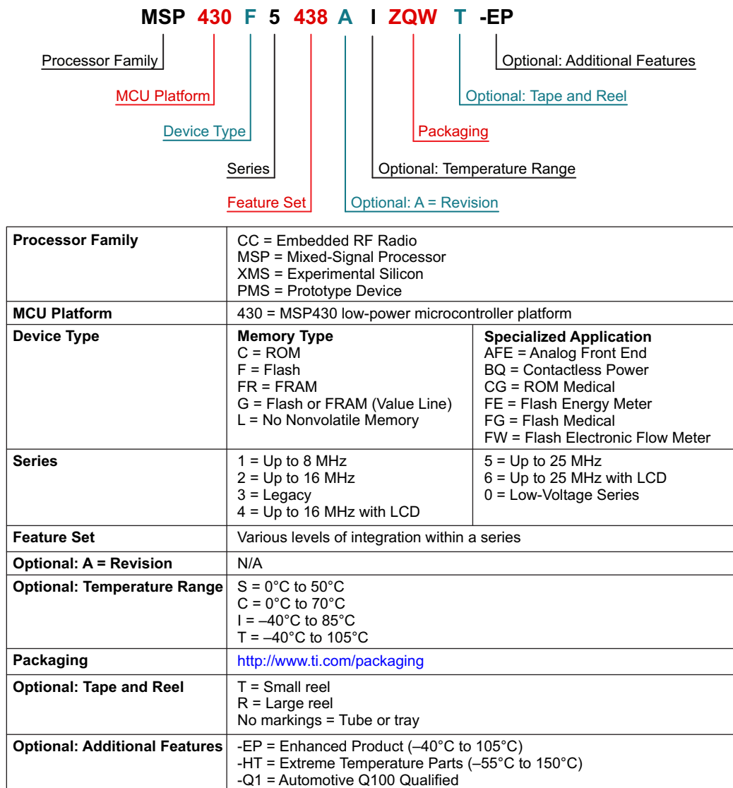
Figure 8-1. Device Nomenclature
