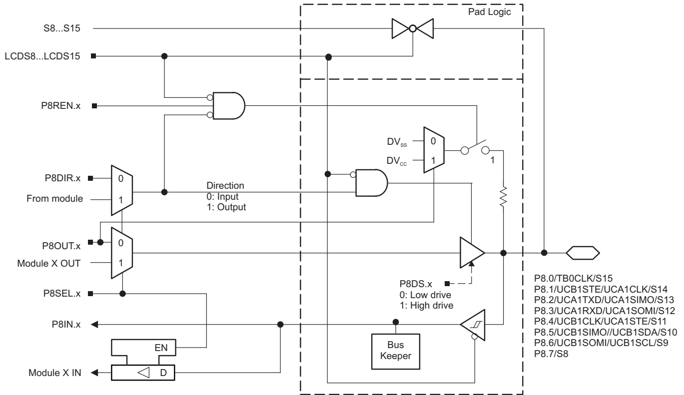
Figure 6-22. Port P8 (P8.0 to P8.7) Diagram
