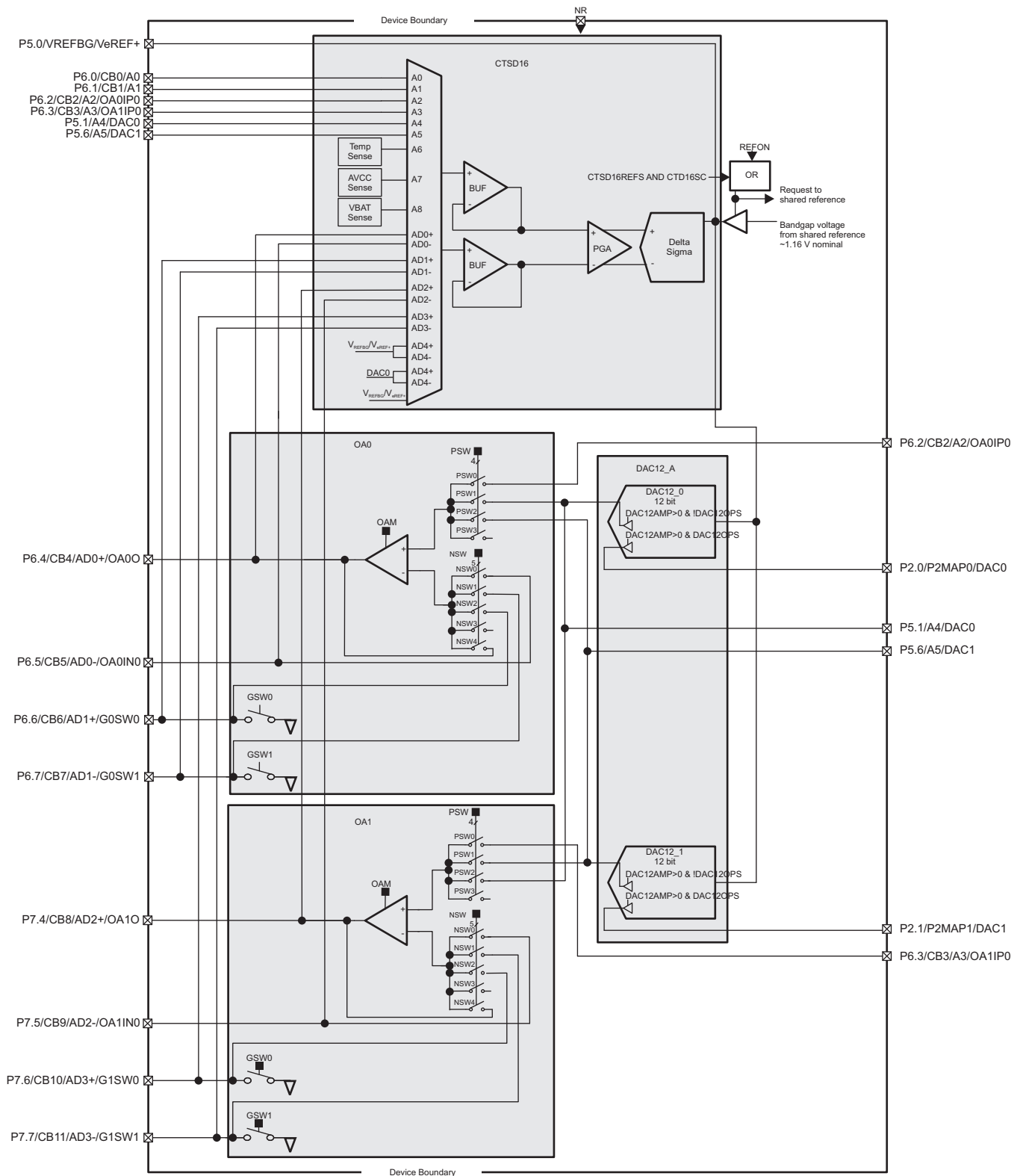
Figure 6-2. Signal Chain
