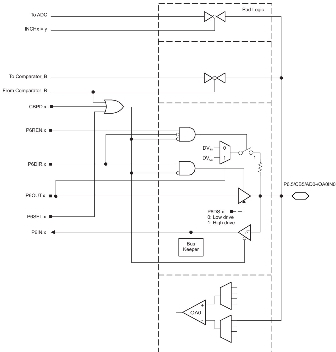
Figure 6-13. Port P6 (P6.5) Diagram
