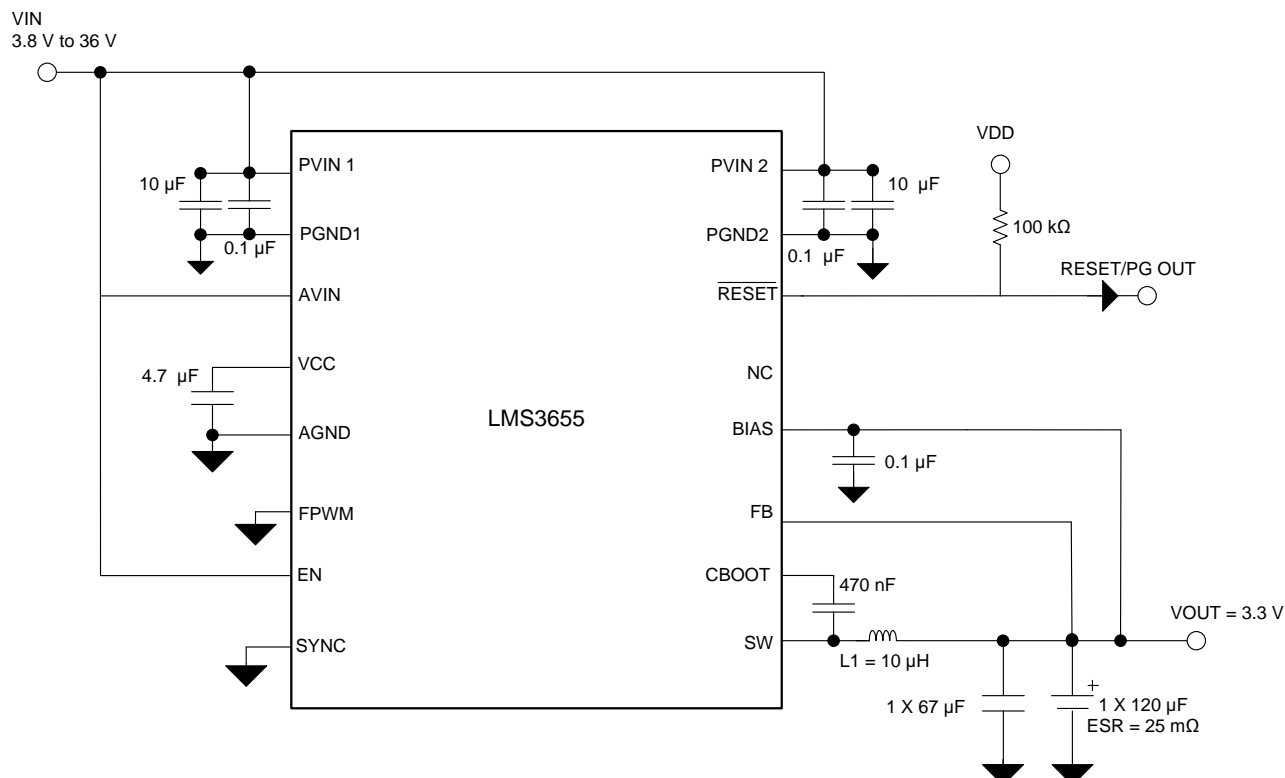
Figure 35. Fixed 3.3-V, 5.5-A Output Power Supply
