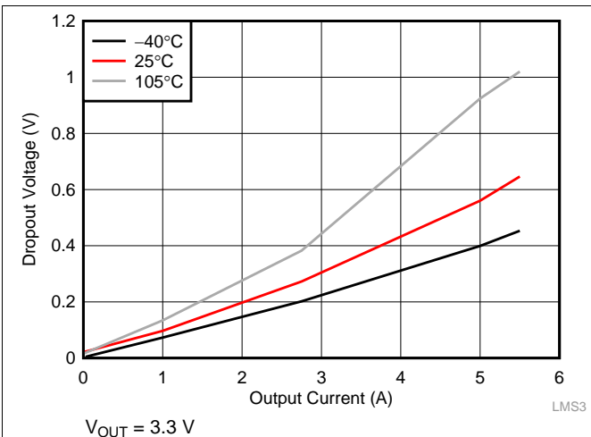
Figure 42. Dropout for -3% Regulation
