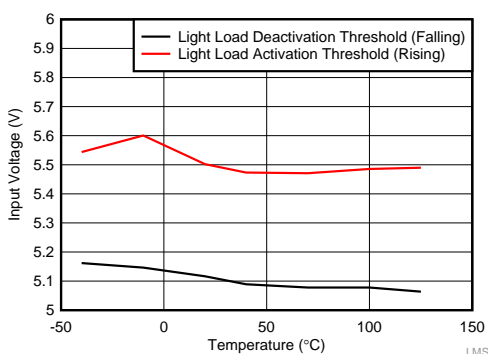
Figure 17. Input Voltage for Mode Change — 5-V Output, 10-μH Inductor
