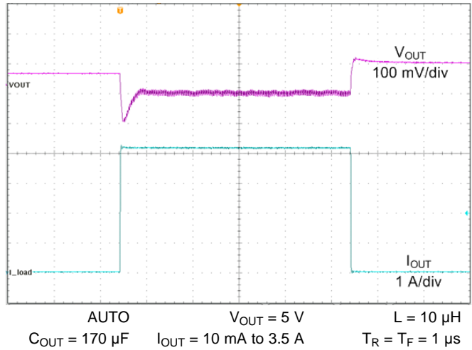
Figure 33. Load Transients
