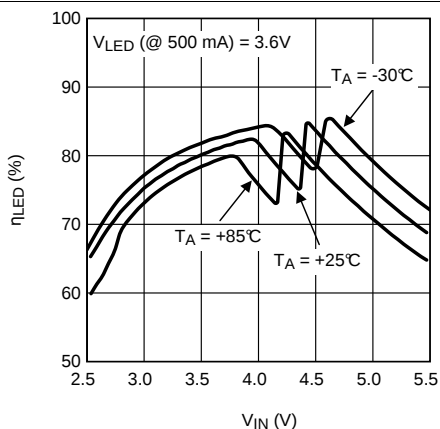
Figure 53. LED Efficiency vs Input Voltage
