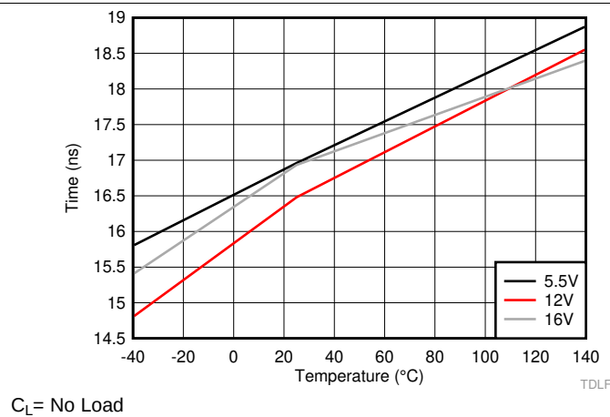
Figure 31. LO Falling Propagation Delay (TDLF)
