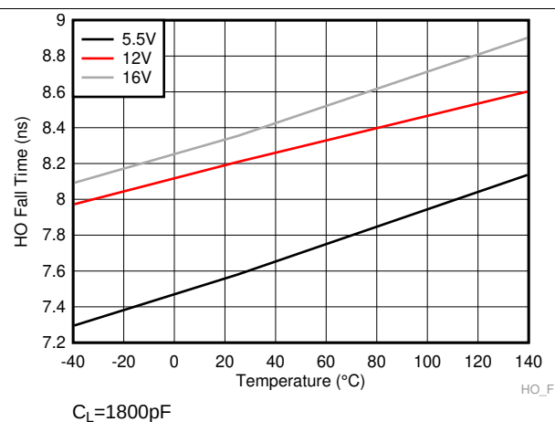
Figure 25. HO Fall Time
