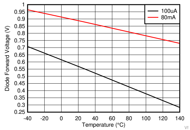
Figure 16. Boot Diode Forward Voltage Drop
