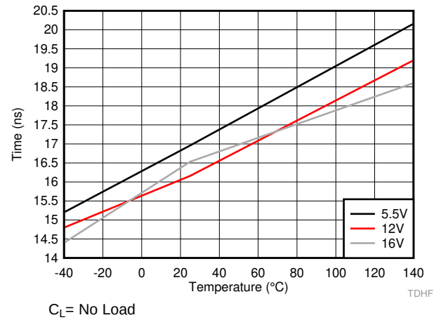
Figure 29. HO Falling Propagation Delay (TDHF)
