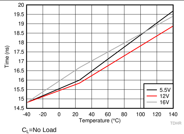
Figure 28. HO Rising Propagation Delay (TDHR)
