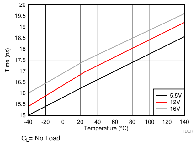
Figure 30. LO Rising Propagation Delay (TDLR)
