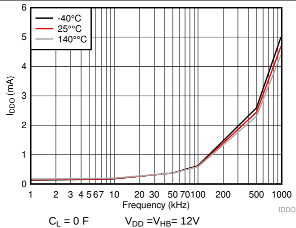
Figure 3. VDD Operating Current
