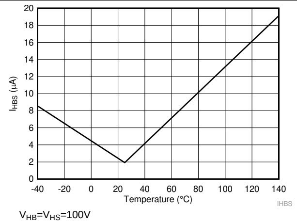
Figure 6. HB to VSS Quiescent Current
