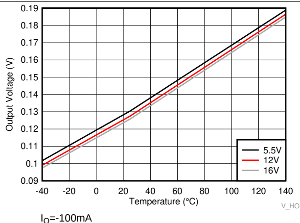
Figure 21. HO High Output Voltage ( V_{HOH} )
