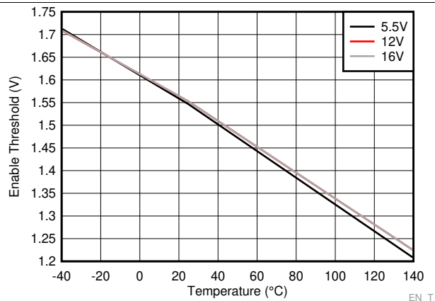
Figure 10. Enable Threshold
