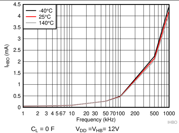
Figure 4. HB Operating Current
