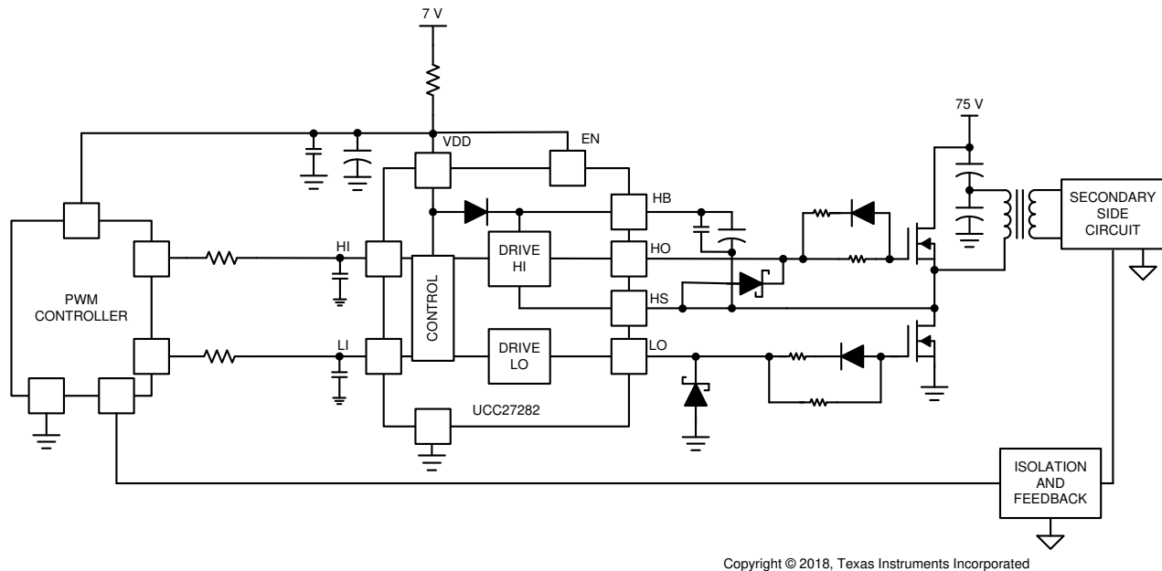
Figure 33. Typical Application
