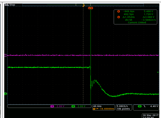
Figure 36. HO Fall Time
