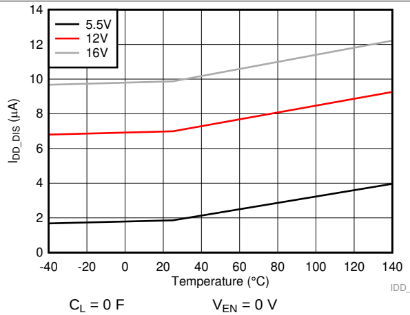
Figure 5. VDD Current When Disabled
