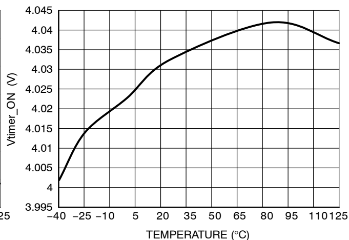
Figure 19. Fault Timer Ending Voltage (V timer(on) )
