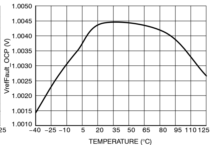
Figure 21. OCP Fault Reference (V ref_Fault_OCP )
