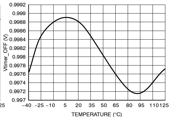
Figure 17. Fault tmr. Reset Voltage (V timer(off) )
