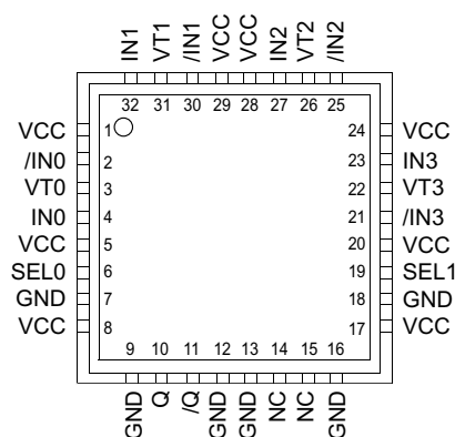
32-Pin MLF®
