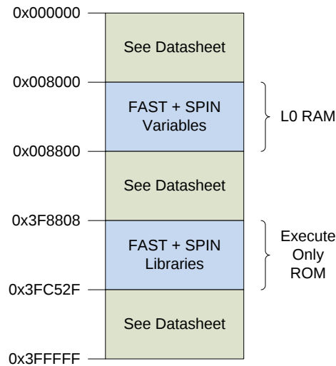
Figure 8. F2805xF Allocated Memory for InstaSPIN-FOC Library
