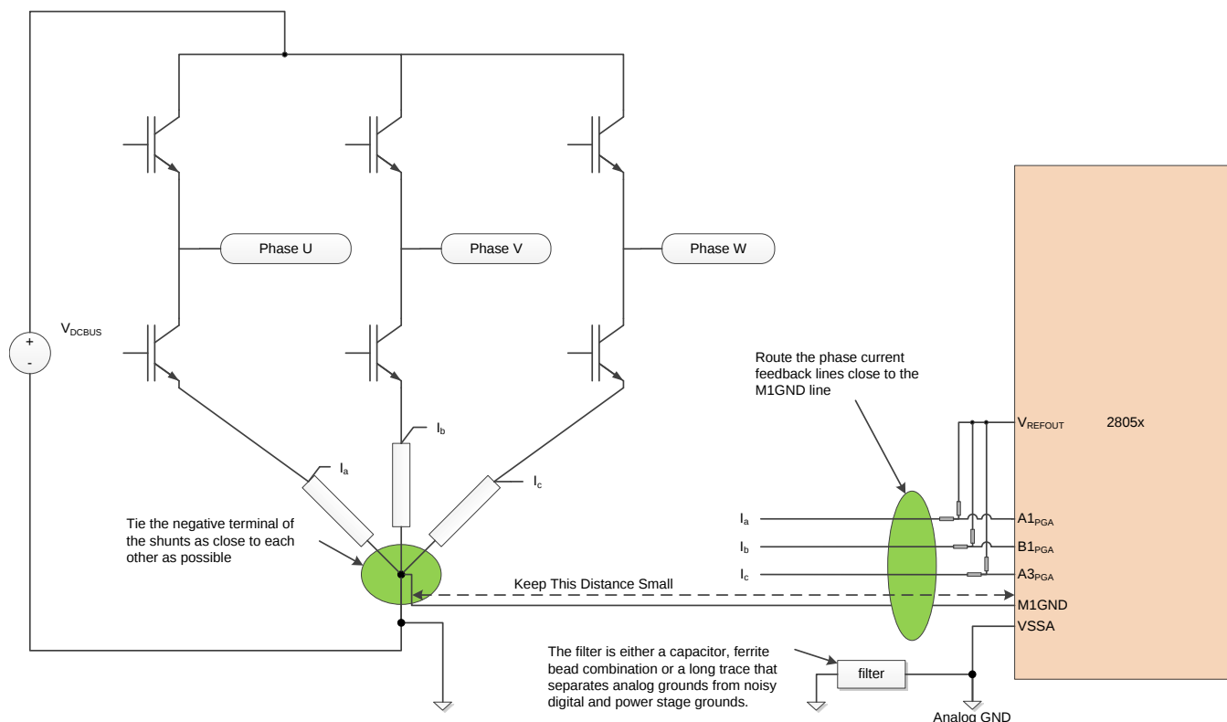
Figure 10. Current Signal Routing Directly to PGAs With Single-Ended Connections
