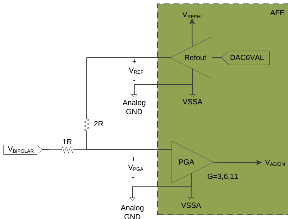
Figure 12. Using the AFE's Built-In Voltage Reference For Measuring a Bipolar Signal
