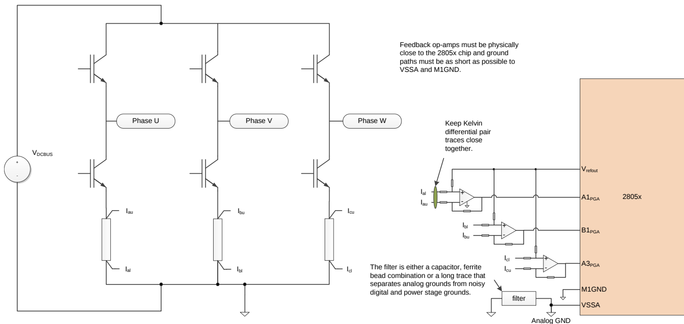
Figure 11. Feedback of Phase Currents Using External Differential Amplifiers
