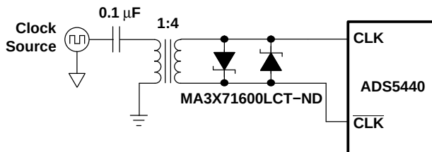
Figure 39. Differential Clock
